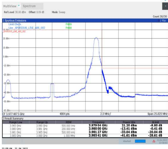
1-N77-3700-3980--30-15-H-2-DFT-PI2BPSK-Edge_1R B_Right-1@37-Ant1-PASS-see graph
