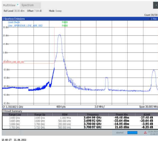
1-N77-3700-3980--30-20-L-4-CP-QPSK-Edge_1RB_L eft-1@0-Ant1-PASS-see graph
