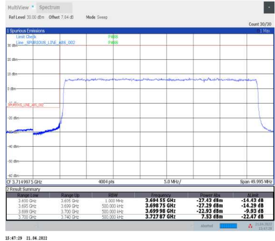
1-N77-3700-3980--30-40-L-3-DFT-PI2BPSK-Outer _Full-100@0-Ant1-PASS-see graph
