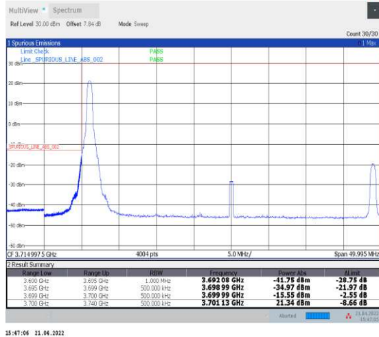
1-N77-3700-3980--30-40-L-1-DFT-PI2BPSK-Edge_1R B_Left-1@0-Ant1-PASS-see graph
