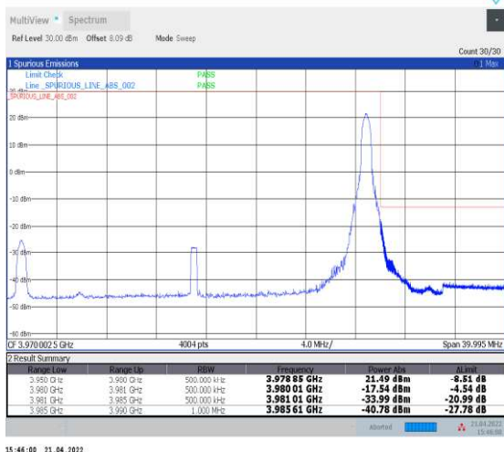
1-N77-3700-3980--30-30-H-5-CP-QPSK-Edge_1RB_R ight-1@77-Ant1-PASS-see graph
