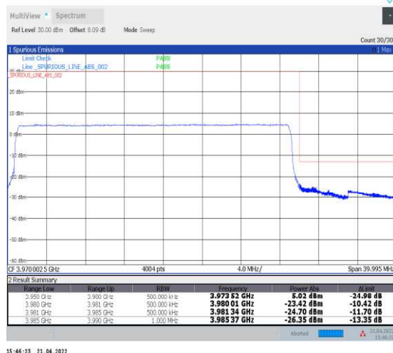
1-N77-3700-3980--30-30-H-6-CP-QPSK-Outer_Fu ll-78@0-Ant1-PASS-see graph
