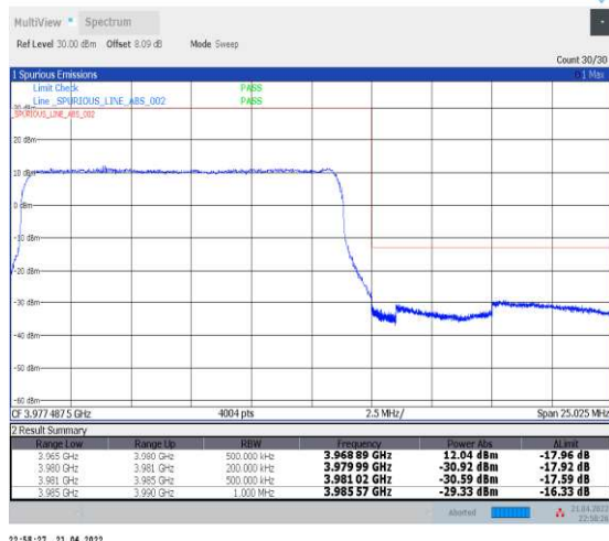
1-N77-3700-3980--30-15-H-3-DFT-PI2BPSK-Outer _Full-36@0-Ant1-PASS-see graph
