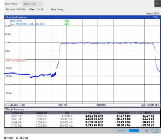
1-N77-3700-3980--30-20-L-3-DFT-PI2BPSK-Outer _Full-50@0-Ant1-PASS-see graph
