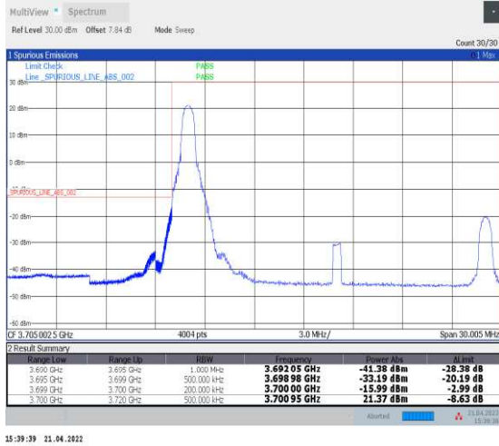
1-N77-3700-3980--30-20-L-1-DFT-PI2BPSK-Edge_1R B_Left-1@0-Ant1-PASS-see graph
