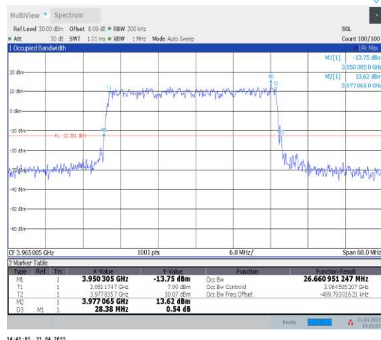
1-N77-3700-3980--30-30-H-3-DFT-16QAM-Outer_Fu ll-75@0-Ant1-26.665-28.380-≤30-PASS
