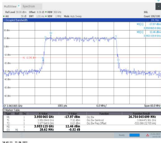
1-N77-3700-3980--30-30-H-4-DFT-64QAM-Outer_F ull-75@0-Ant1-26.756-28.620-≤30-PASS
