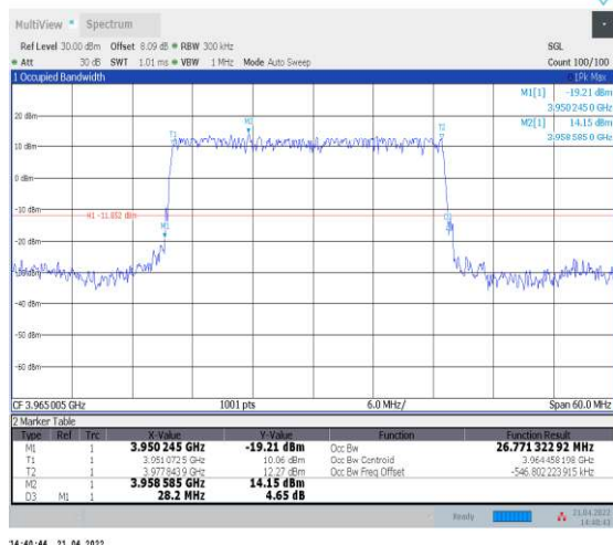
1-N77-3700-3980--30-30-H-2-DFT-PI2BPSK-Outer_ Full-75@0-Ant1-26.774-28.200-≤30-PASS
