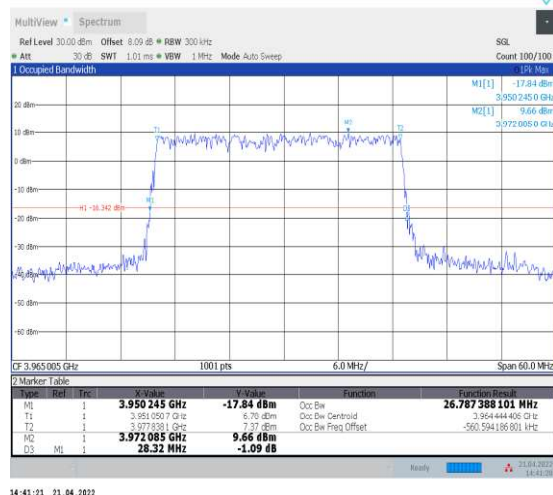
1-N77-3700-3980--30-30-H-5-DFT-256QAM-Outer_F ull-75@0-Ant1-26.788-28.320-≤30-PASS
