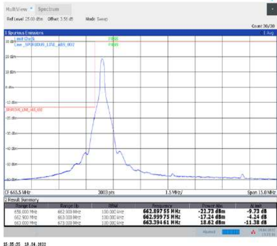
1-N71--15-10-L-1-DFT-PI2BPSK-Edge_1RB_Left-1@0-Ant1-PASS-see graph
