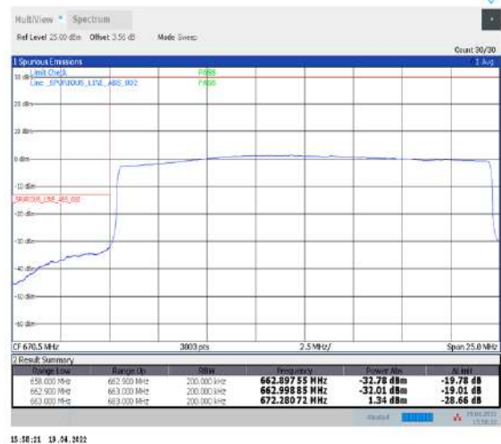
1-N71--15-20-L-6-CP-QPSK-Outer_Full-106@0-Ant1-PASS-see graph
