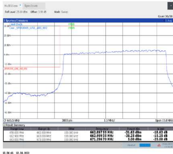
1-N71--15-10-L-3-DFT-PI2BPSK-Outer_Full-50@0-Ant1-PASS-see graph
