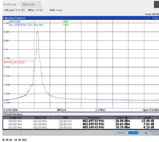
1-N71--15-20-L-1-DFT-PI2BPSK-Edge_1RB_Left-1@0-Ant1-PASS-see graph
