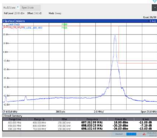
1-N71--15-15-H-5-CP-QPSK-Edge_1RB_Right-1@78-Ant1-PASS-see graph
