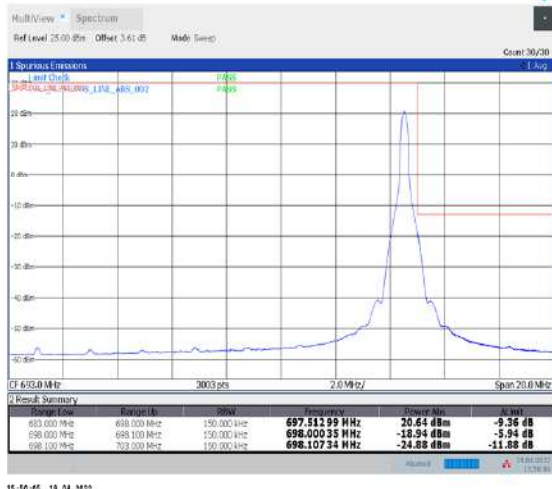
1-N71--15-15-H-2-DFT-PI2BPSK-Edge_1RB_Right-1@78-Ant1-PASS-see graph
