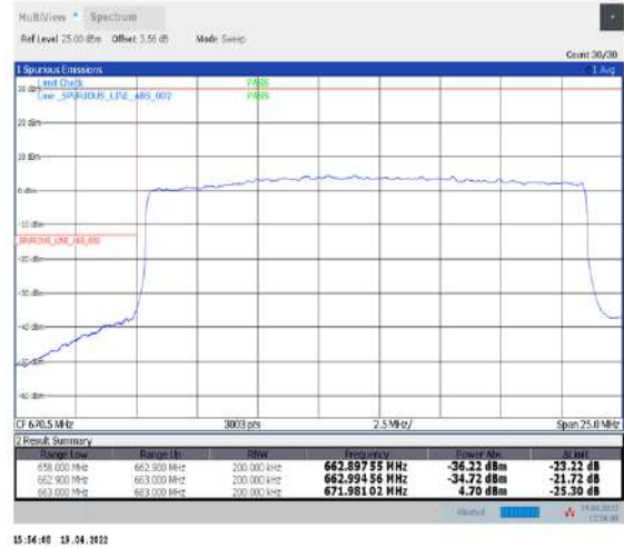
1-N71--15-20-L-3-DFT-PI2BPSK-Outer_Full-100@0-Ant1-PASS-see graph
