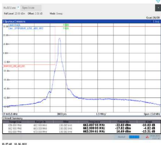
1-N71--15-10-L-4-CP-QPSK-Edge_1RB_Left-1@0-Ant1-PASS-see graph
