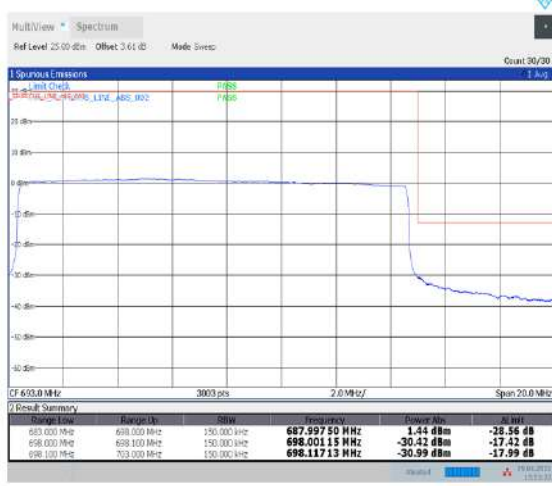
1-N71--15-15-H-6-CP-QPSK-Outer_Full-79@0-Ant1-PASS-see graph
