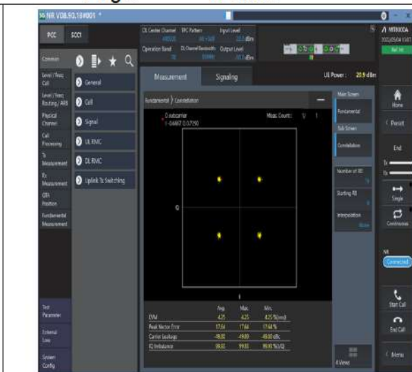
1-N70-PC3-15-15-M-6-CP-QPSK-Outer_Full-79@0-Ant1-see graph-PASS
