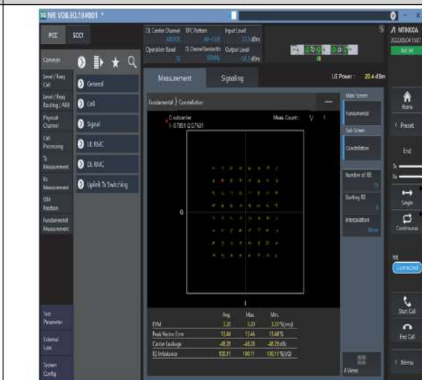
1-N70-PC3-15-15-M-8-CP-64QAM-Outer_Full-79@0-Ant1-see graph-PASS
