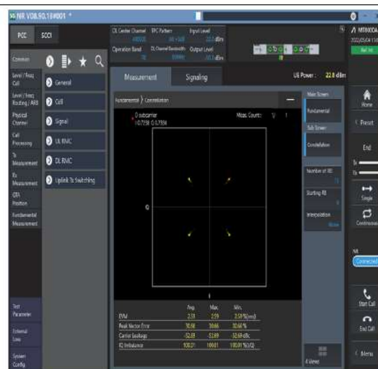
1-N70-PC3-15-15-M-2-DFT-QPSK-Outter_Full-75@0-Ant1-see graph-PASS
