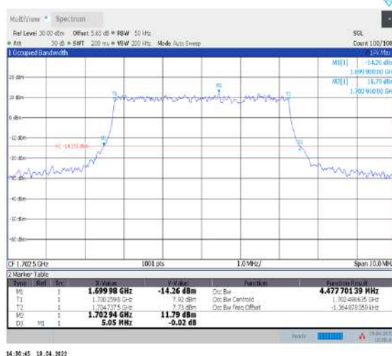
1-N70--15-5-M-3-DFT-16QAM-Outer_Full-25@0- Ant1-4.478-5.050-≤5-PASS
