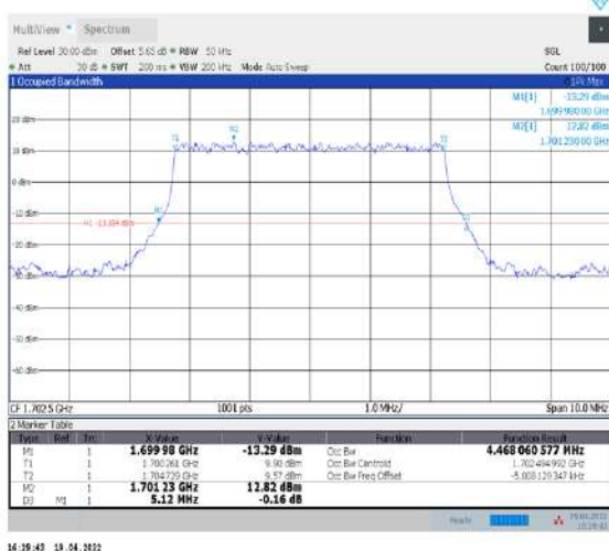
1-N70--15-5-M-2-DFT-PI2BPSK-Outer_Full-25@0- Ant1-4.468-5.120-≤5-PASS
