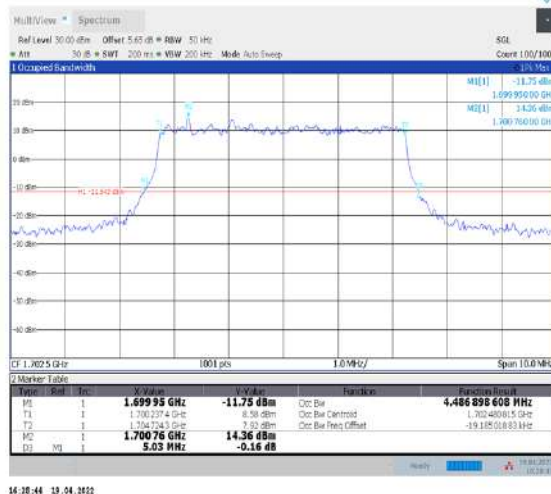
1-N70--15-5-M-1-DFT-QPSK-Outer_Full-25@0- Ant1-4.487-5.030-≤5-PASS
