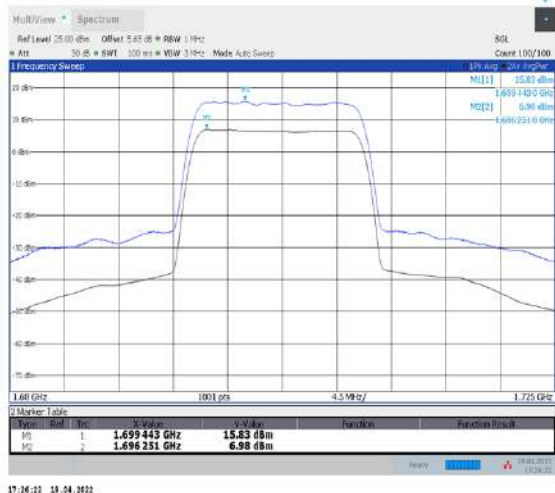
1-N70--15-15-L-1-DFT-256QAM-Outer_Full-75@0- Ant1-8.85-100%-0.00-8.85-PASS-≤13
