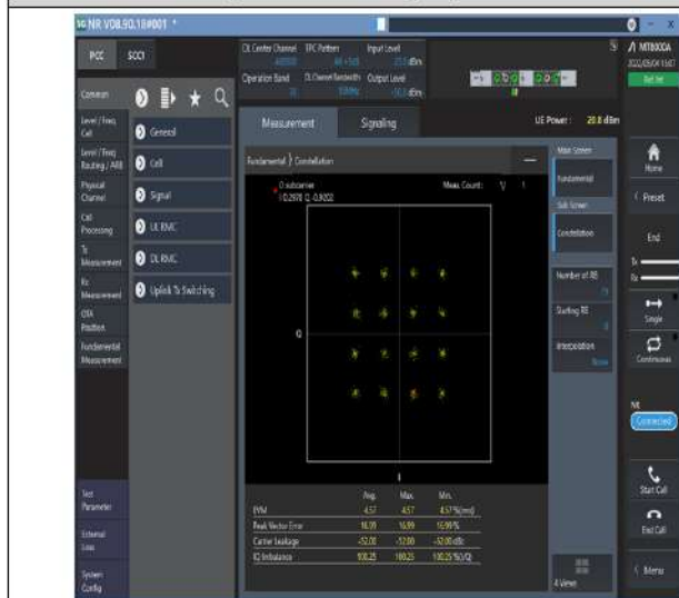
1-N70-PC3-15-15-M-7-CP-16QAM-Outer_Full-79@0-Ant1-see graph-PASS
