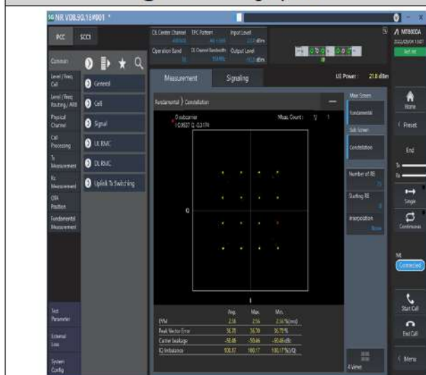
1-N70-PC3-15-15-M-3-DFT-16QAM-Outter_Full-75@0-Ant1-see graph-PASS
