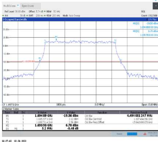
1-N70--15-5-L-9-CP-256QAM-Outer_Full-25@0- Ant1-4.494-5.200-≤5-PASS
