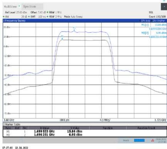
1-N70--15-15-M-1-DFT-256QAM-Outer_Full-75@0- Ant1-8.89-100%-0.00-8.89-PASS-≤13
