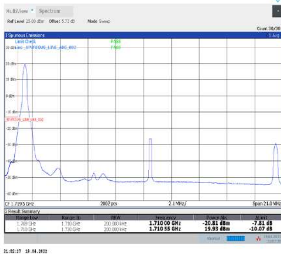
1-N66-PC3-15-20-L-4-CP-QPSK-Edge_1RB_Left-1@0-Ant1-seegraph-PASS-see graph
