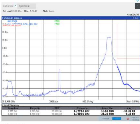
1-N66-PC3-15-5-H-5-CP-QPSK-Edge_1RB_Right-1@24-Ant1-seegraph-PASS-see graph
