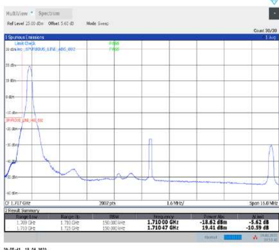
1-N66-PC3-15-15-L-4-CP-QPSK-Edge_1RB_Left-1@0-Ant1-seegraph-PASS-see graph
