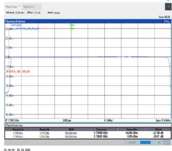
1-N66-PC3-15-40-L-6-CP-QPSK-Outer_Full-216@0-Ant1-seegraph-PASS-see graph
