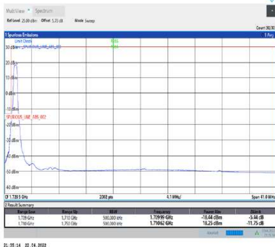
1-N66-PC3-15-40-L-4-CP-QPSK-Edge_1RB_Left-1@0-Ant1-seegraph-PASS-see graph
