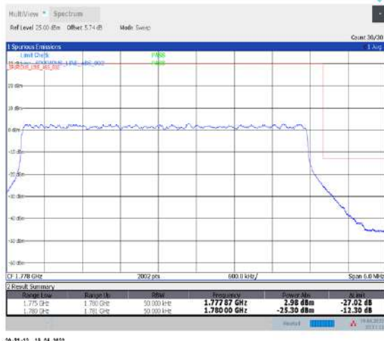
1-N66-PC3-15-5-H-3-DFT-PI2BPSK-Outer_Full-25@0-Ant1-seegraph-PASS-see graph
