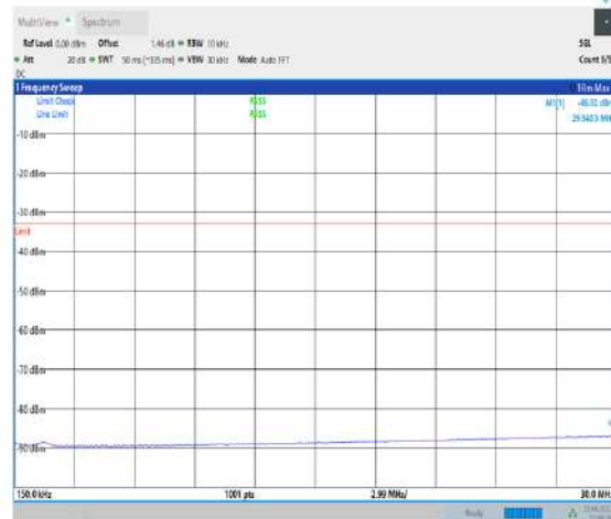
1-N66-PC3-15-40-H-1-DFT-PI2BPSK- Inner_1RB_Left-1@1-0.15-30-Ant1--86.92--33-PASS
