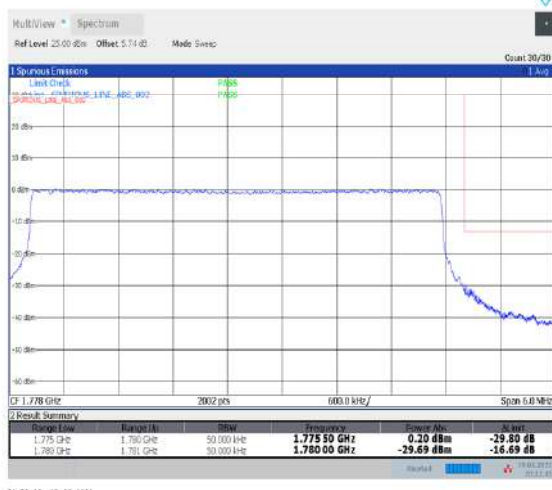
1-N66-PC3-15-5-H-6-CP-QPSK-Outer_Full-25@0-Ant1-seegraph-PASS-see graph
