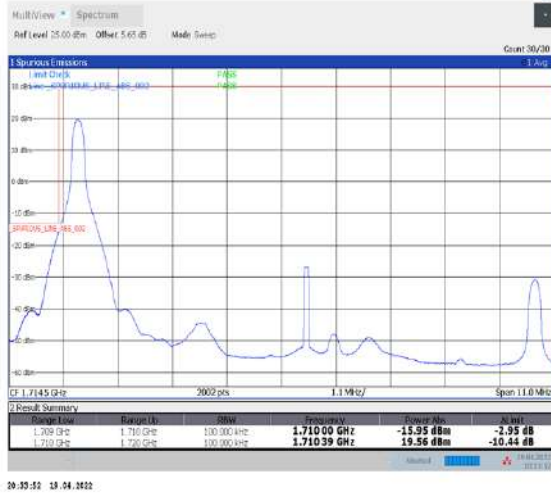
1-N66-PC3-15-10-L-1-DFT-PI2BPSK-Edge_1RB_Left-1@0-Ant1-seegraph-PASS-see graph
