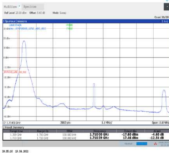
1-N66-PC3-15-10-L-4-CP-QPSK-Edge_1RB_Left-1@0-Ant1-seegraph-PASS-see graph
