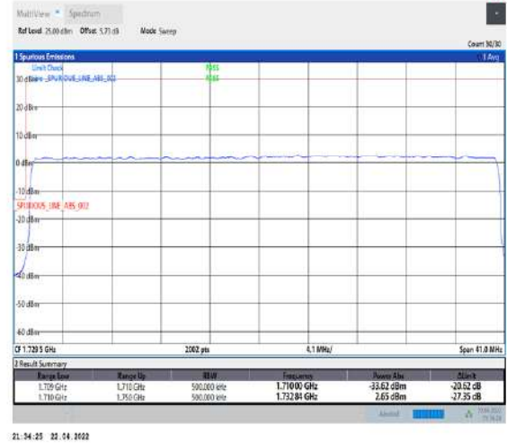
1-N66-PC3-15-40-L-3-DFT-PI2BPSK-Outer_Full-216@0-Ant1-seegraph-PASS-see graph
