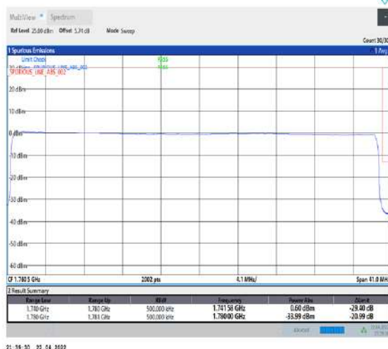
1-N66-PC3-15-40-H-6-CP-QPSK-Outer_Full-216@0-Ant1-seegraph-PASS-see graph
