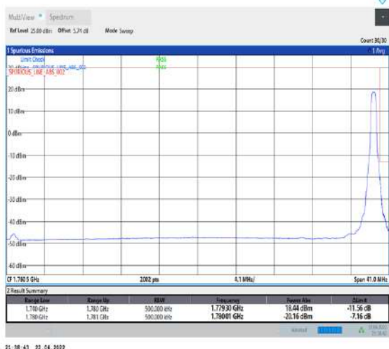
1-N66-PC3-15-40-H-5-CP-QPSK-Edge_1RB_Right-1@215-Ant1-seegraph-PASS-see graph
