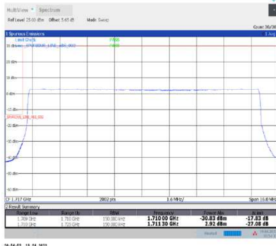
1-N66-PC3-15-15-L-3-DFT-PI2BPSK-Outer_Full-75@0-Ant1-seegraph-PASS-see graph
