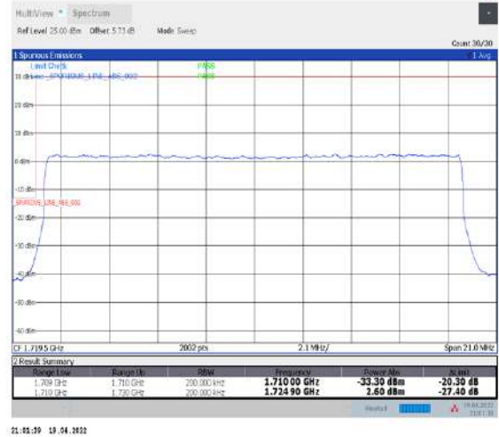
1-N66-PC3-15-20-L-3-DFT-PI2BPSK-Outer_Full-100@0-Ant1-seegraph-PASS-see graph
