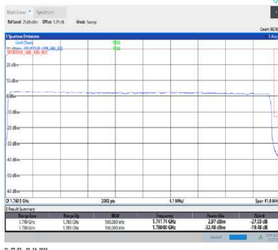
1-N66-PC3-15-40-H-3-DFT-PI2BPSK-Outer_Full-216@0-Ant1-seegraph-PASS-see graph
