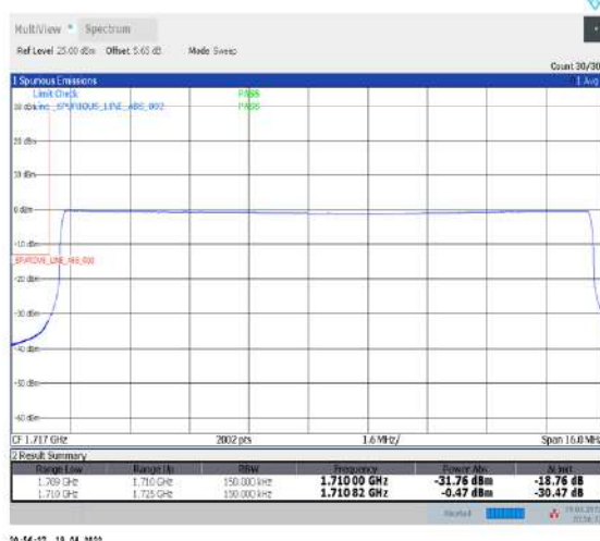
1-N66-PC3-15-15-L-6-CP-QPSK-Outer_Full-79@0-Ant1-seegraph-PASS-see graph
