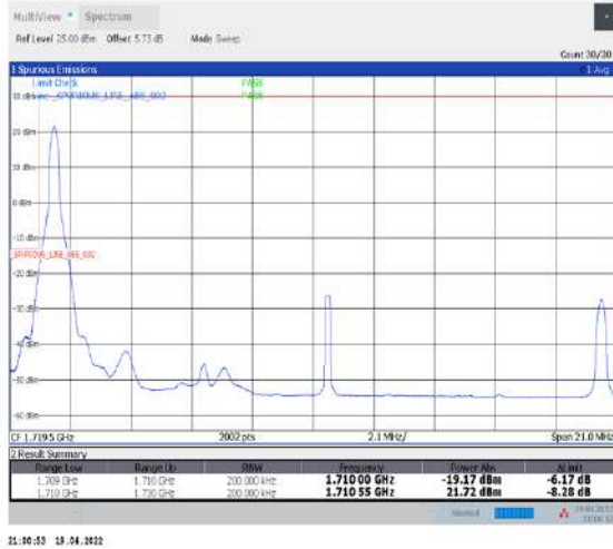
1-N66-PC3-15-20-L-1-DFT-PI2BPSK-Edge_1RB_Left-1@0-Ant1-seegraph-PASS-see graph
