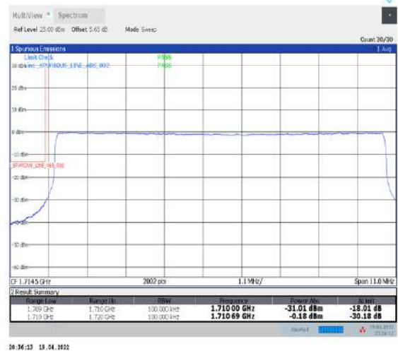
1-N66-PC3-15-10-L-6-CP-QPSK-Outer_Full-52@0-Ant1-seegraph-PASS-see graph
