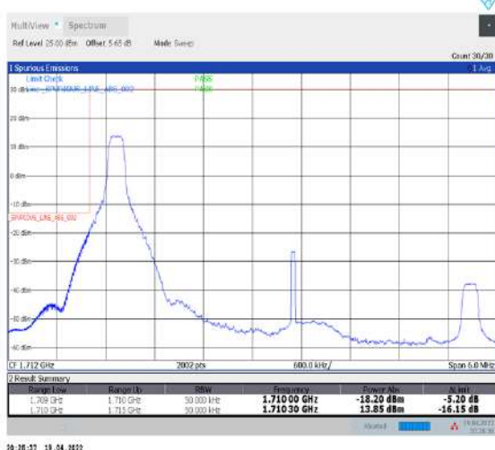
1-N66-PC3-15-5-L-4-CP-QPSK-Edge_1RB_Left-1@0-Ant1-seegraph-PASS-see graph
