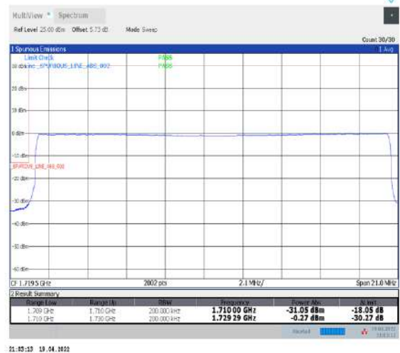
1-N66-PC3-15-20-L-6-CP-QPSK-Outer_Full-106@0-Ant1-seegraph-PASS-see graph
