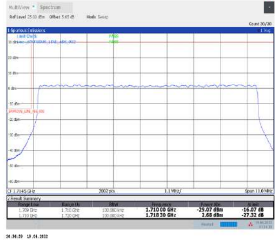
1-N66-PC3-15-10-L-3-DFT-PI2BPSK-Outer_Full-50@0-Ant1-seegraph-PASS-see graph
