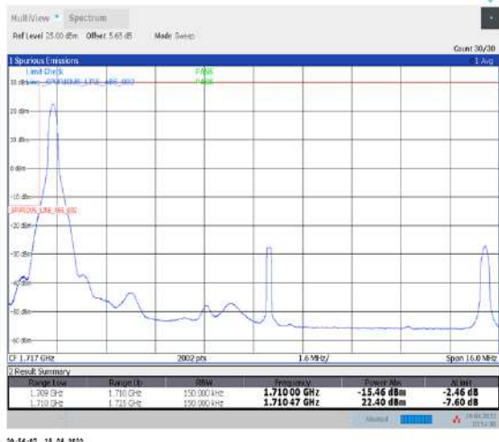
1-N66-PC3-15-15-L-1-DFT-PI2BPSK-Edge_1RB_Left-1@0-Ant1-seegraph-PASS-see graph
