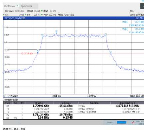
1-N66-PC3-15-5-L-4-DFT-64QAM-Outer_Full-25@0- Ant1-4.474-5.140-≤5-PASS
