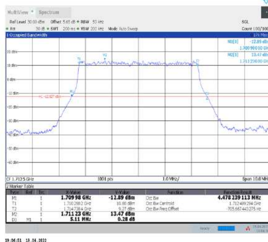
1-N66-PC3-15-5-L-2-DFT-PI2BPSK-Outer_Full- 25@0-Ant1-4.478-5.110-≤5-PASS
