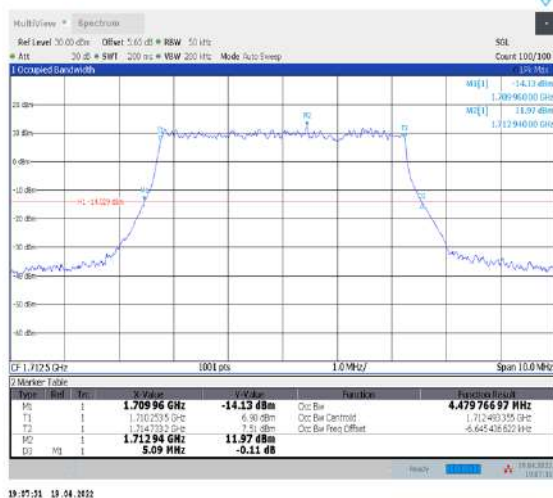
1-N66-PC3-15-5-L-3-DFT-16QAM-Outer_Full-25@0- Ant1-4.48-5.090-≤5-PASS
