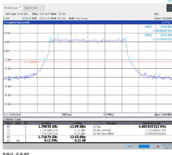
1-N66-PC3-15-5-L-1-DFT-QPSK-Outer_Full-25@0- Ant1-4.481-5.120-≤5-PASS
