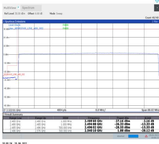
1-N41--30-80-L-6-CP-QPSK-Outer_Full-217@0-Ant1-PASS-see graph
