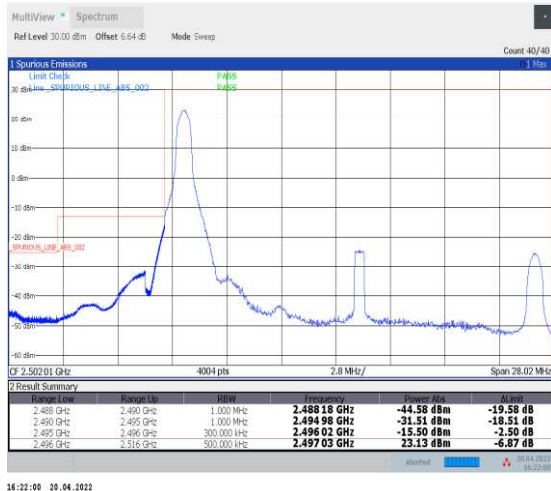
1-N41--30-20-L-4-CP-QPSK-Edge_1RB_Left-1@0-Ant1-PASS-see graph
