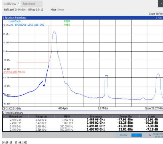
1-N41--30-20-L-1-DFT-PI2BPSK-Edge_1RB_Left-1@0-Ant1-PASS-see graph
