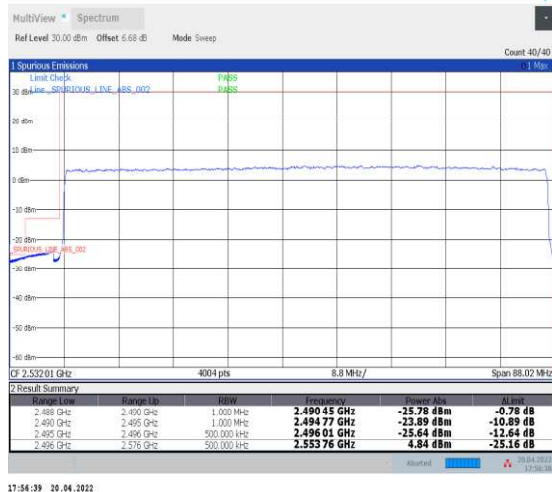
1-N41--30-80-L-3-DFT-PI2BPSK-Outer_Full-216@0-Ant1-PASS-see graph
