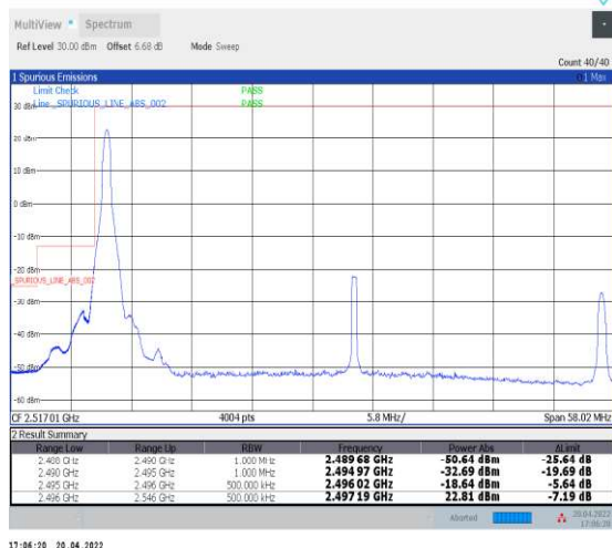
1-N41--30-50-L-4-CP-QPSK-Edge_1RB_Left-1@0-Ant1-PASS-see graph
