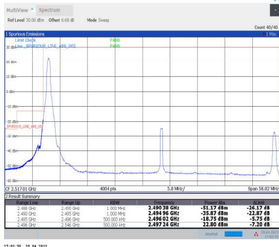
1-N41--30-50-L-1-DFT-PI2BPSK-Edge_1RB_Left-1@0-Ant1-PASS-see graph
