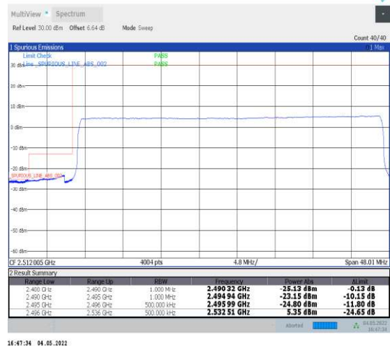
1-N41--30-40-L-6-CP-QPSK-Outer_Full-106@0-Ant1-PASS-see graph
