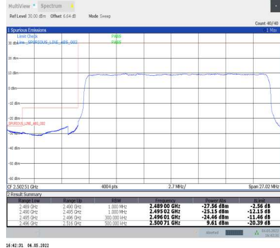
1-N41--30-20-L-3-DFT-PI2BPSK-Outer_Full-50@0-Ant1-PASS-see graph
