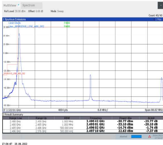
1-N41--30-80-L-1-DFT-PI2BPSK-Edge_1RB_Left-1@0-Ant1-PASS-see graph
