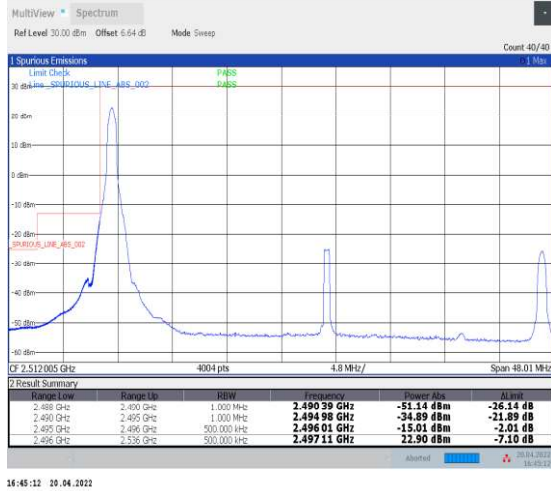
1-N41--30-40-L-1-DFT-PI2BPSK-Edge_1RB_Left-1@0-Ant1-PASS-see graph
