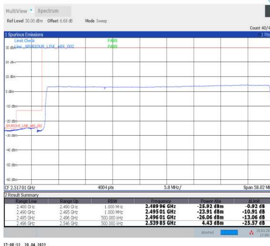
1-N41--30-50-L-6-CP-QPSK-Outer_Full-133@0-Ant1-PASS-see graph
