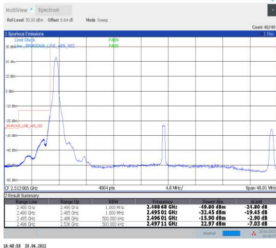
1-N41--30-40-L-4-CP-QPSK-Edge_1RB_Left-1@0-Ant1-PASS-see graph
