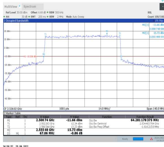
1-N41--30-70-L-1-DFT-QPSK-Outer_Full-180@0-Ant 1-64.281-67.060-≤70-PASS
