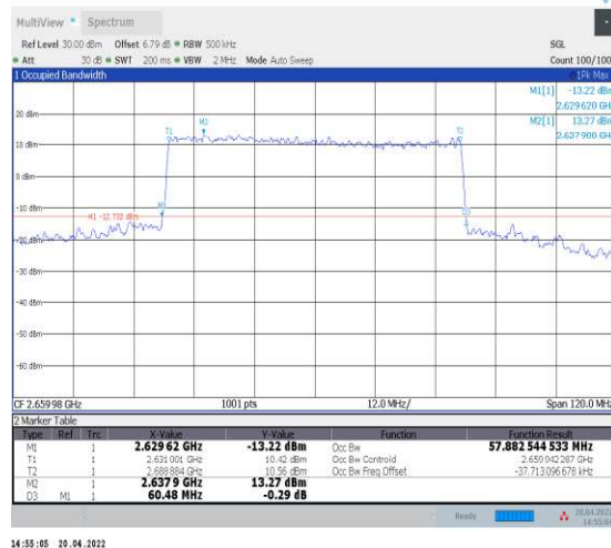
1-N41--30-60-H-8-CP-64QAM-Outer_Full-162@0-An t1-57.883-60.480-≤60-PASS
