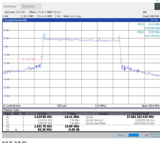
1-N41--30-60-H-9-CP-256QAM-Outer_Full-162@0-A nt1-57.861-60.360-≤60-PASS
