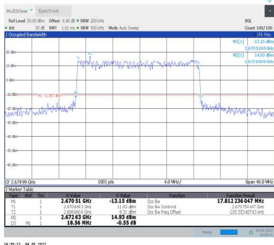
1-N41--30-20-H-3-DFT-16QAM-Outer_Full-50@0-An t1-17.812-18.560-≤20-PASS
