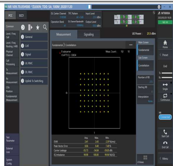
1-N41-30-100-M-8-CP-64QAM-Outer_Full-273@0-Ant1-see graph-PASS
