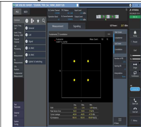
1-N41--30-100-M-6-CP-QPSK-Outer_Full-273@0-Ant1-see graph-PASS
