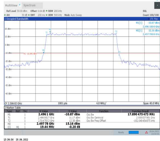
1-N41--30-20-L-4-DFT-64QAM-Outer_Full-50@0-An t1-17.89-19.440-≤20-PASS
