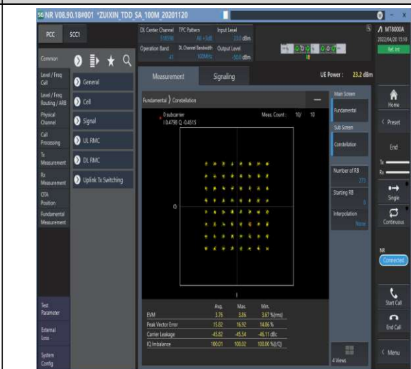
1-N41--30-100-M-8-CP-64QAM-Outer_Full-273@0-Ant1-see graph-PASS
