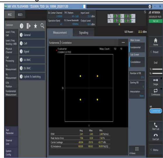
1-N41-30-100-M-6-CP-QPSK-Outer_Full-273@0-Ant1-see graph-PASS
