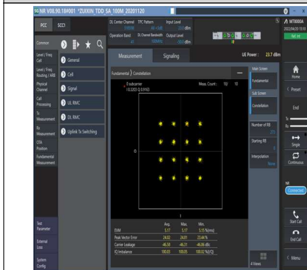
1-N41--30-100-M-7-CP-16QAM-Outer_Full-273@0-Ant1-see graph-PASS
