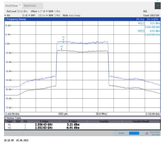
1-N41--30-100-M-2-CP-256QAM-Outer_Full-273@0-Ant1-10.12-100%-0.00-10.12-PASS-≤13
