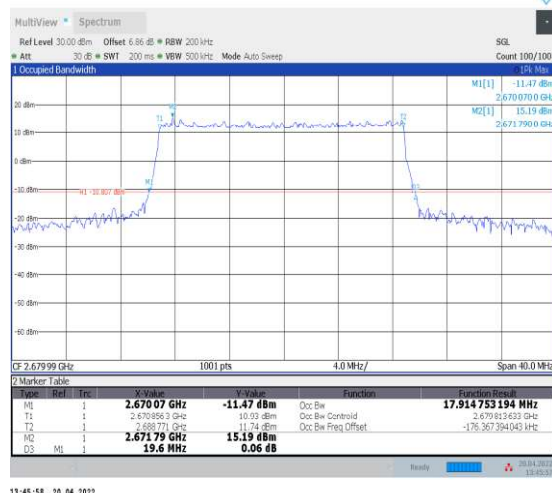
1-N41--30-20-H-4-DFT-64QAM-Outer_Full-50@0-An t1-17.915-19.600-≤20-PASS
