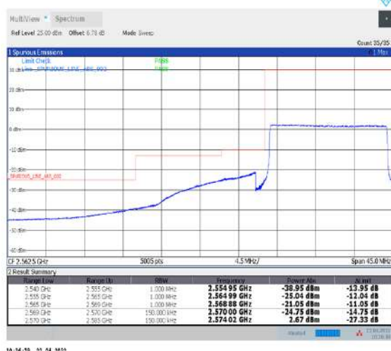
1-N38--30-15-L-6-CP-QPSK-Outer_Full-38@0-Ant1-PASS-see graph
