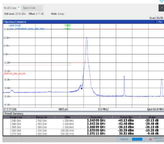
1-N38--30-30-L-4-CP-QPSK-Edge_1RB_Left-1@0-Ant1-PASS-see graph
