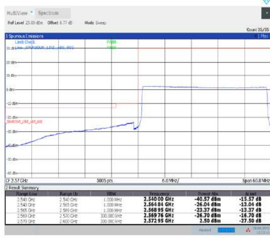
1-N38--30-30-L-6-CP-QPSK-Outer_Full-78@0-Ant1-PASS-see graph
