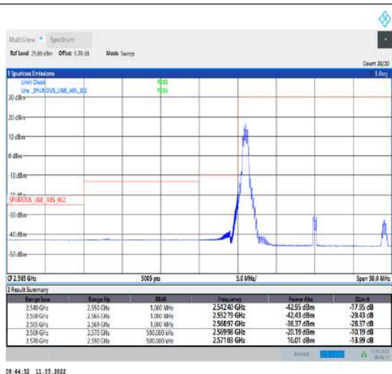
1-N38-PC2-30-20-L-4-CP-QPSK-Edge_1RB_Left-1@0-Ant1-PASS-see graph
