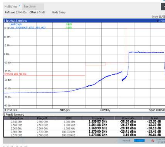
1-N38--30-10-L-6-CP-QPSK-Outer_Full-24@0-Ant1-PASS-see graph
