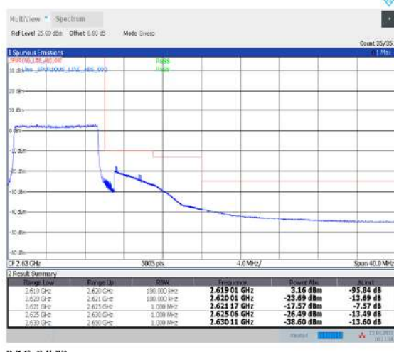
1-N38--30-10-H-6-CP-QPSK-Outer_Full-24@0-Ant1-PASS-see graph
