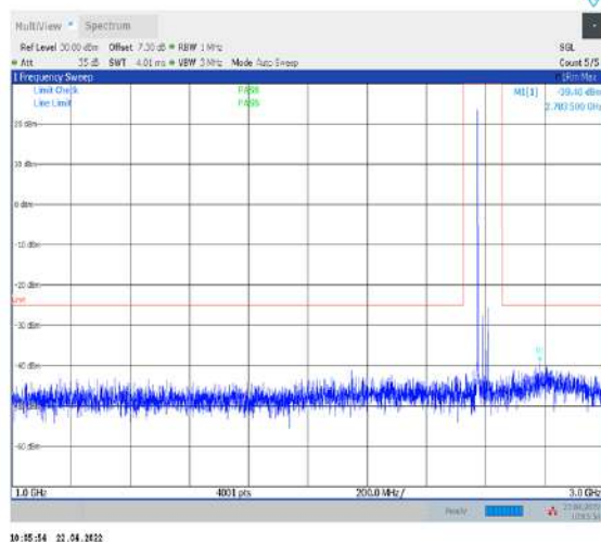
1-N38--30-40-L-1-DFT-PI2BPSK-Inner_1RB_Left- 1@1-1000-3000-Ant1--39.40--25-PASS
