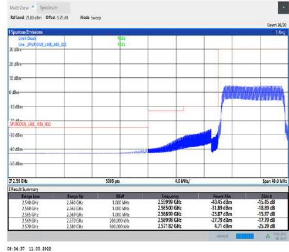
1-N38-PC2-30-10-L-6-CP-QPSK-Outer_Full-24@0-Ant1-PASS-see graph
