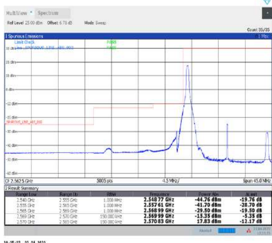
1-N38--30-15-L-4-CP-QPSK-Edge_1RB_Left-1@0-Ant1-PASS-see graph
