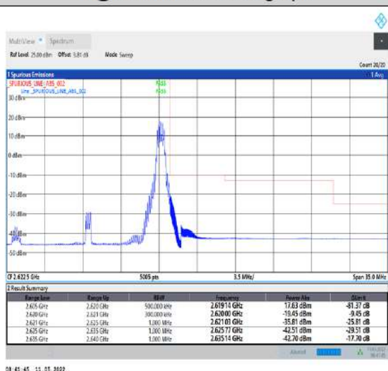
1-N38-PC2-30-15-H-5-CP-QPSK-Edge_1RB_Right- 1@37-Ant1-PASS-see graph
