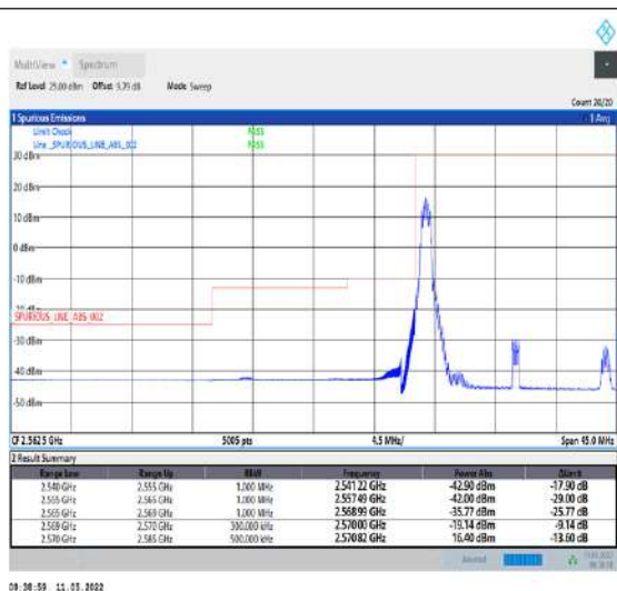
1-N38-PC2-30-15-L-4-CP-QPSK-Edge_1RB_Left- 1@0-Ant1-PASS-see graph
