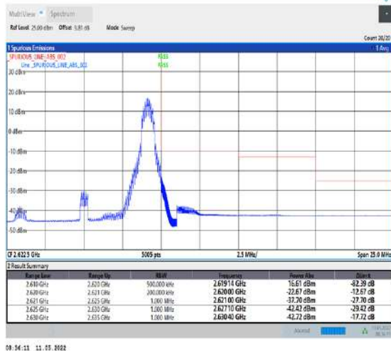
1-N38-PC2-30-10-H-5-CP-QPSK-Edge_1RB_Right-1@23-Ant1-PASS-see graph
