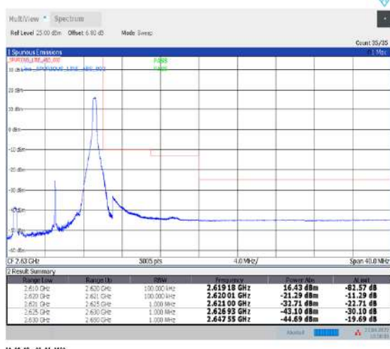
1-N38--30-10-H-5-CP-QPSK-Edge_1RB_Right-1@23-Ant1-PASS-see graph
