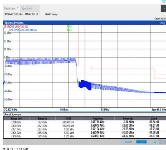
1-N38-PC2-30-30-H-6-CP-QPSK-Outer_Full-78@0-Ant1-PASS-see graph
