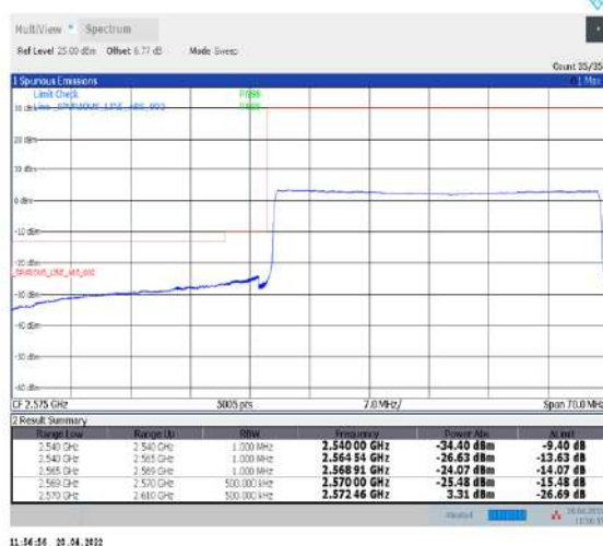
1-N38--30-40-L-6-CP-QPSK-Outer_Full-106@0-Ant1-PASS-see graph
