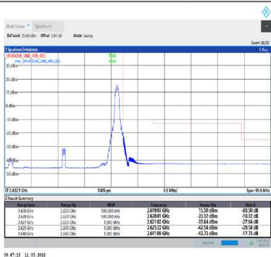
1-N38-PC2-30-20-H-5-CP-QPSK-Edge_1RB_Right-1@50-Ant1-PASS-see graph
