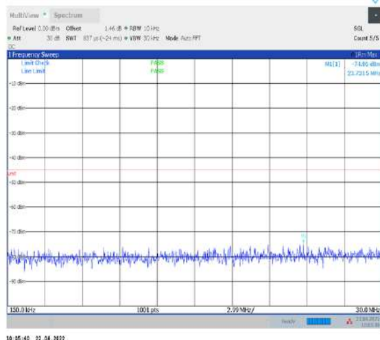
1-N38--30-40-L-1-DFT-PI2BPSK-Inner_1RB_Left- 1@1-0.15-30-Ant1--74.86--45-PASS
