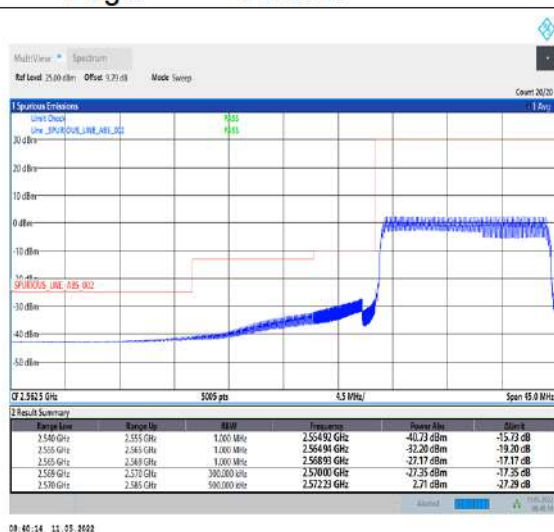
1-N38-PC2-30-15-L-6-CP-QPSK-Outer_Full- 38@0-Ant1-PASS-see graph
