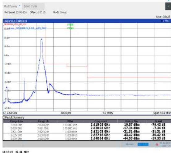
1-N38--30-10-H-2-DFT-PI2BPSK-Edge_1RB_Right-1@23-Ant1-PASS-see graph
