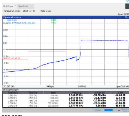
1-N38--30-20-L-6-CP-QPSK-Outer_Full-51@0-Ant1-PASS-see graph
