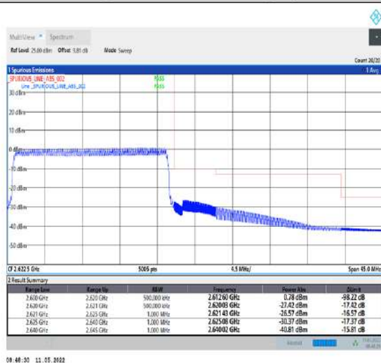
1-N38-PC2-30-20-H-6-CP-QPSK-Outer_Full-51@0-Ant1-PASS-see graph
