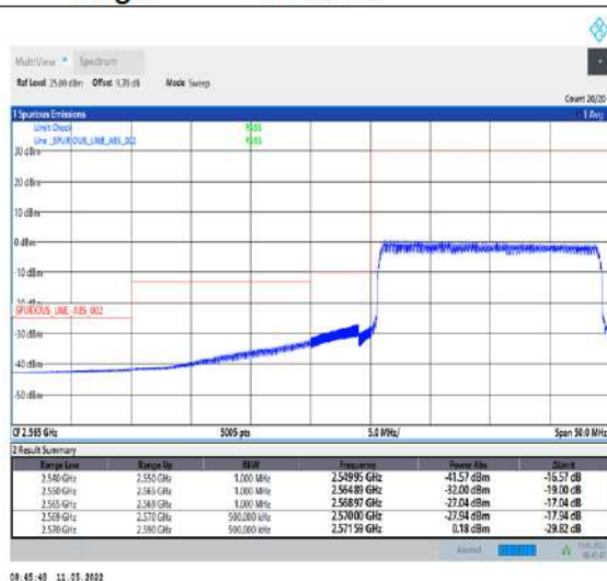
1-N38-PC2-30-20-L-6-CP-QPSK-Outer_Full-51@0-Ant1-PASS-see graph
