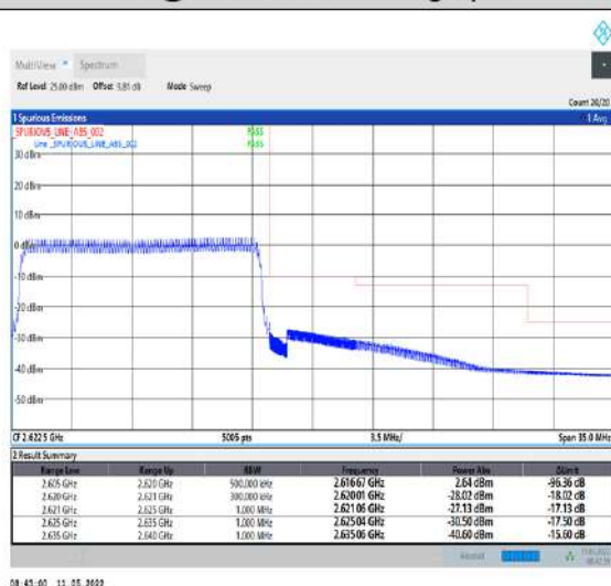
1-N38-PC2-30-15-H-6-CP-QPSK-Outer_Full- 38@0-Ant1-PASS-see graph
