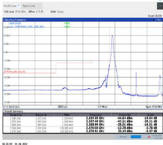
1-N38--30-15-L-1-DFT-PI2BPSK-Edge_1RB_Left-1@0-Ant1-PASS-see graph
