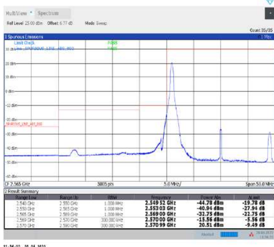
1-N38--30-20-L-4-CP-QPSK-Edge_1RB_Left-1@0-Ant1-PASS-see graph
