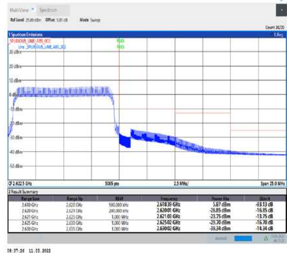
1-N38-PC2-30-10-H-6-CP-QPSK-Outer_Full-24@0-Ant1-PASS-see graph
