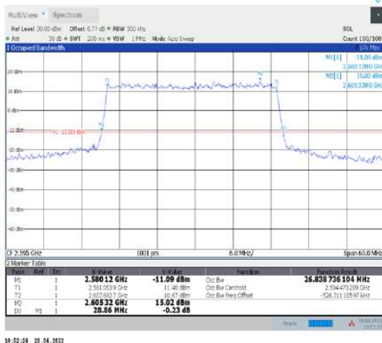
1-N38--30-30-M-1-DFT-QPSK-Outer_Full-75@0-Ant1-26.839-28.860-≤30-PASS
