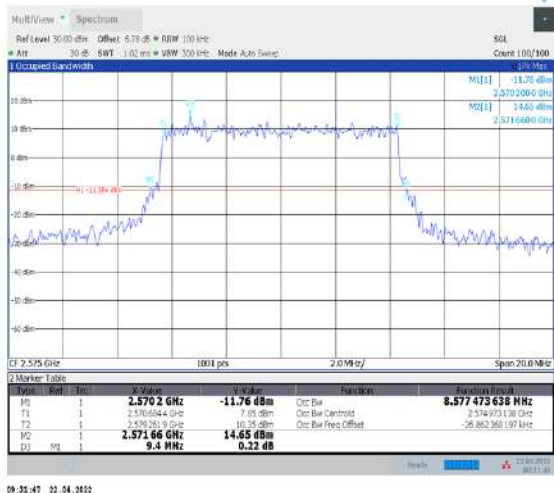
1-N38--30-10-L-1-DFT-QPSK-Outer_Full-24@0- Ant1-8.577-9.400-≤10-PASS
