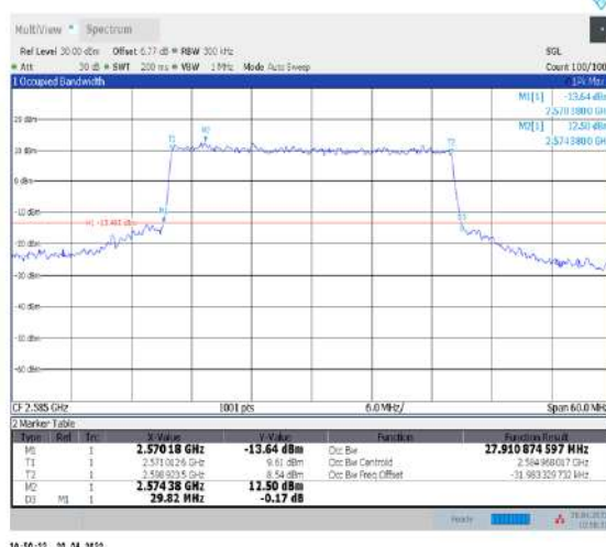
1-N38-30-30-L-7-CP-16QAM-Outer_Full-78@0-Ant1-27.911-29.820-≤30-PASS
