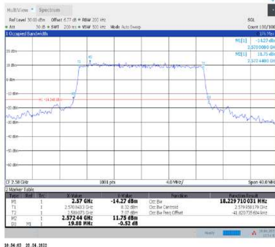
1-N38--30-20-L-8-CP-64QAM-Outer_Full-51@0-Ant1-18.23-19.880-≤20-PASS
