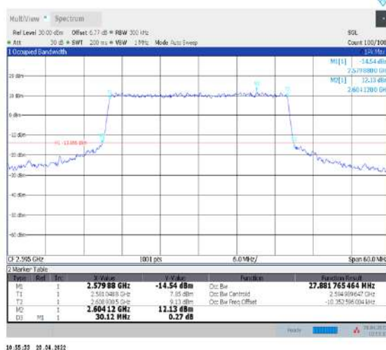
1-N38--30-30-M-6-CP-QPSK-Outer_Full-78@0-Ant1-27.882-30.120-≤30-PASS
