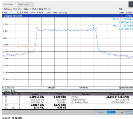
1-N38--30-30-M-3-DFT-16QAM-Outer_Full-75@0-Ant1-26.885-28.800-≤30-PASS
