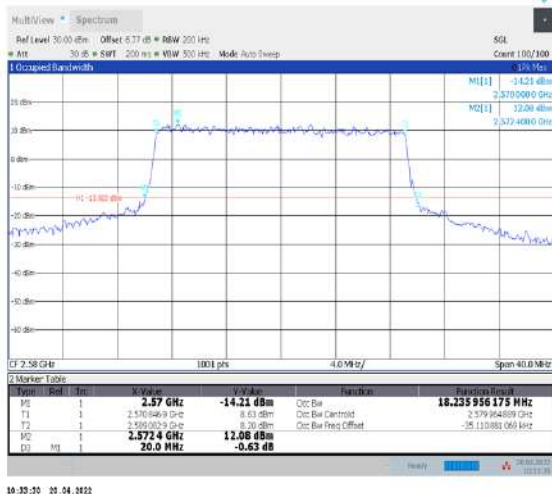
1-N38--30-20-L-7-CP-16QAM-Outer_Full-51@0-Ant1-18.236-20.000-≤20-PASS
