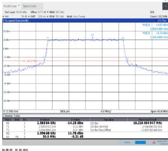
1-N38--30-20-M-6-CP-QPSK-Outer_Full-51@0-Ant1-18.226-20.000-≤20-PASS
