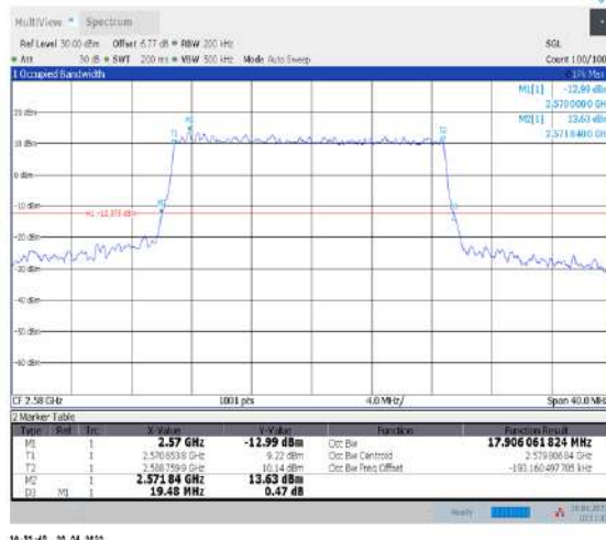
1-N38--30-20-L-4-DFT-64QAM-Outer_Full-50@0-Ant1-17.906-19.480-≤20-PASS
