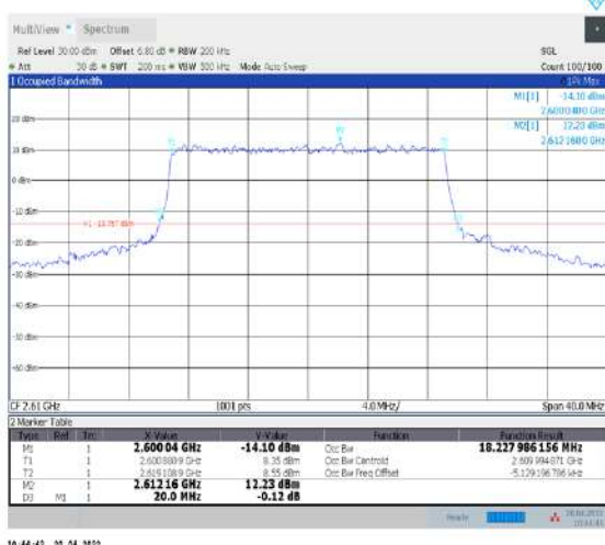
1-N38--30-20-H-7-CP-16QAM-Outer_Full-51@0-Ant1-18.228-20.000-≤20-PASS
