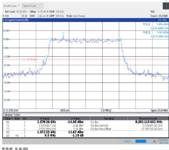
1-N38--30-10-L-3-DFT-16QAM-Outer_Full-24@0- Ant1-8.592-9.500-≤10-PASS
