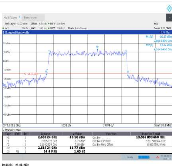
1-N38--30-15-H-8-CP-64QAM-Outer_Full-38@0-Ant1-13.568-14.400-≤15-PASS
