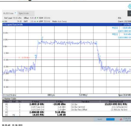
1-N38--30-15-H-9-CP-256QAM-Outer_Full-38@0-Ant1-13.524-14.850-≤15-PASS
