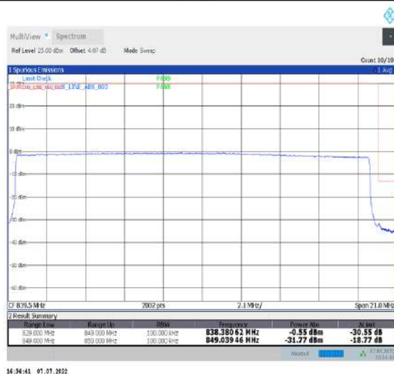
1-N26-824-849--15-20-H-3-DFT-PI2BPSK-Outer_Full-100@0-Ant1-seegraph-PASS-see graph
