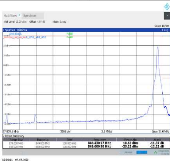
1-N26-824-849--15-20-H-5-CP-QPSK-Edge_1RB_Right-1@105-Ant1-seegraph-PASS-see graph
