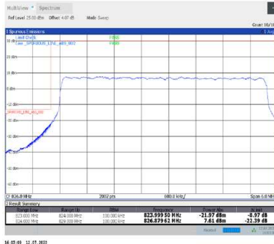
1-N26-824-849--15-5-L-3-DFT-PI2BPSK-Outer_Full-25@0-Ant1-seegraph-PASS-see graph
