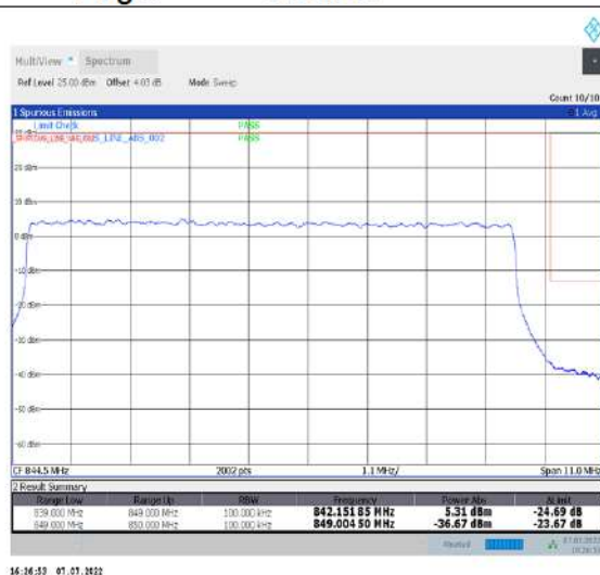
1-N26-824-849--15-10-H-3-DFT-PI2BPSK-Outer_Full-50@0-Ant1-seegraph-PASS-see graph
