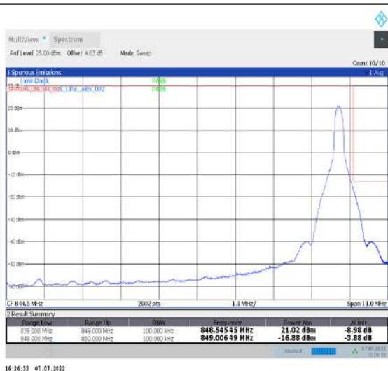
1-N26-824-849--15-10-H-2-DFT-PI2BPSK-Edge_1RB_Right-1@51-Ant1-seegraph-PASS-see graph
