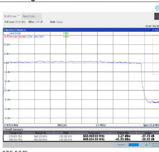
1-N26-824-849--15-20-H-3-DFT-PI2BPSK-Outer_Full-100@0-Ant1-seegraph-PASS-see graph
