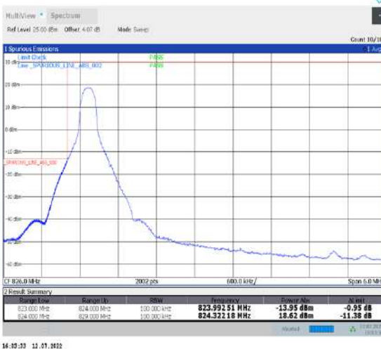
1-N26-824-849--15-5-L-4-CP-QPSK-Edge_1RB_Left-1@0-Ant1-seegraph-PASS-see graph
