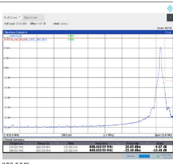
1-N26-824-849--15-20-H-2-DFT-PI2BPSK-Edge_1RB_Right-1@105-Ant1-seegraph-PASS-see graph
