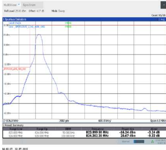
1-N26-824-849--15-5-L-1-DFT-PI2BPSK-Edge_1RB_Left-1@0-Ant1-seegraph-PASS-see graph
