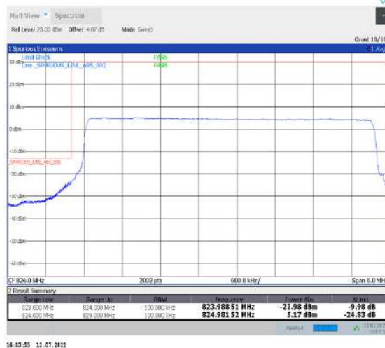
1-N26-824-849--15-5-L-6-CP-QPSK-Outer_Full-25@0-Ant1-seegraph-PASS-see graph
