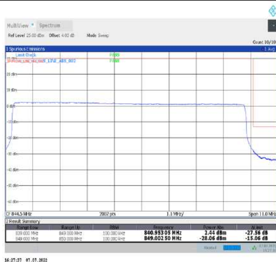
1-N26-824-849--15-10-H-6-CP-QPSK-Outer_Full-52@0-Ant1-seegraph-PASS-see graph
