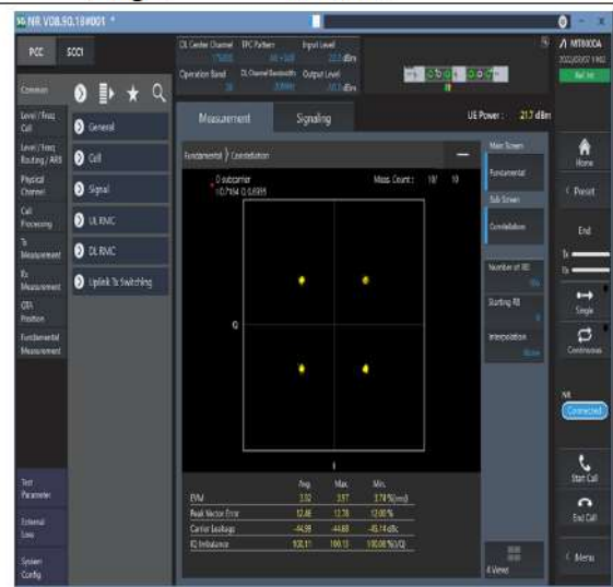
1-N26-824-849--15-20-M-6-CP-QPSK-Outer_Full-106@0-Ant1-see graph-PASS
