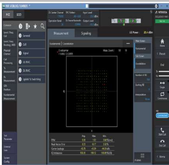
1-N26-824-849--15-20-M-5-DFT-256QAM-Outer_Full-100@0-Ant1-see graph-PASS
