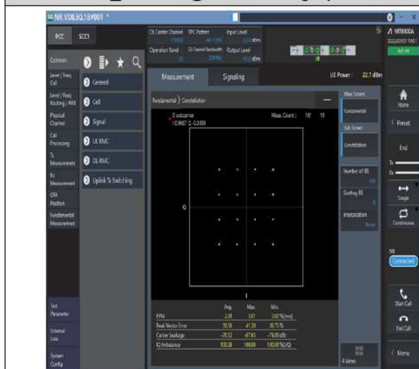
1-N26-824-849--15-20-M-3-DFT-16QAM-Outer_Full-100@0-Ant1-see graph-PASS
