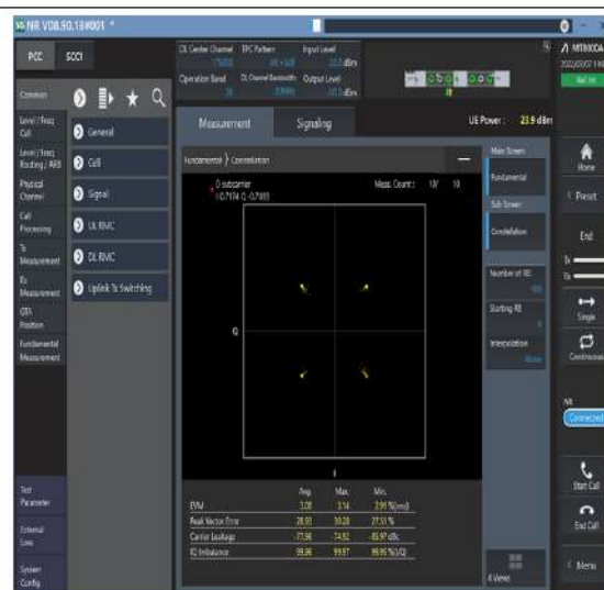
1-N26-824-849--15-20-M-2-DFT-QPSK-Outer_Full-100@0-Ant1-see graph-PASS
