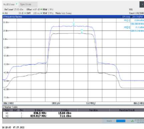
1-N26-824-849--15-20-M-1-DFT-256QAM-Outer_Full-100@0-Ant1-8.73-100%-0.00-8.73-PASS-≤13
