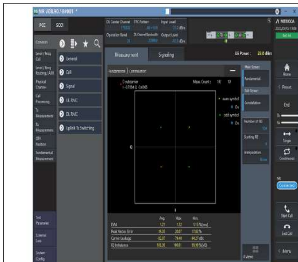
1-N26-824-849--15-20-M-1-DFT-PI2BPSK-Outer_Full-100@0-Ant1-see graph-PASS
