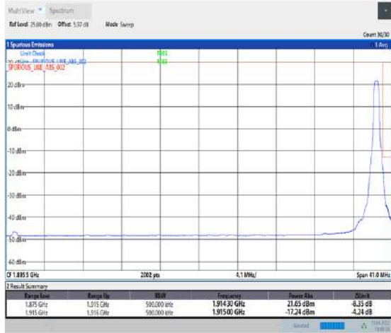
1-N25--15-40-H-2-DFT-PI2BPSK-Edge_1RB_Right-1@215-Ant1-seegraph-PASS-see graph
