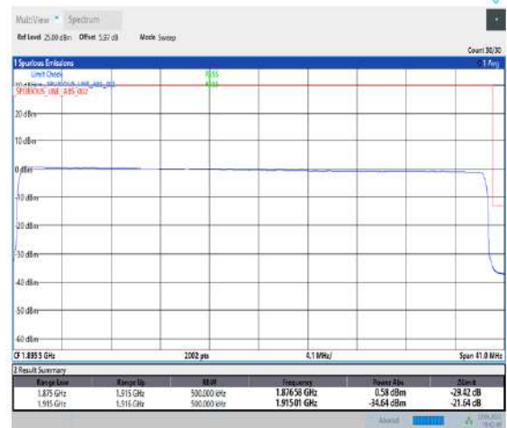
1-N25--15-40-H-6-CP-QPSK-Outer_Full-216@0-Ant1-seegraph-PASS-see graph
