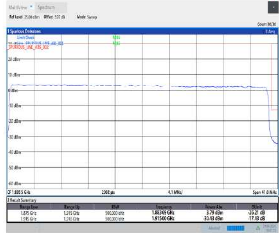
1-N25--15-40-H-3-DFT-PI2BPSK-Outer_Full-216@0-Ant1-seegraph-PASS-see graph
