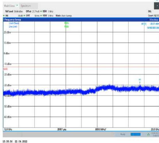
1-N25--15-40-H-1-DFT-PI2BPSK-Inner_1RB_Left- 1@1-12000-20000-Ant1--28.37--13-PASS
