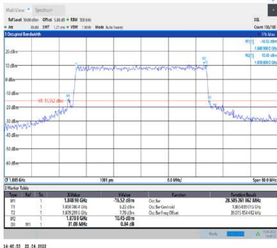
1-N25--15-30-L-6-CP-QPSK-Outer_Full-160@0-Ant1-28.505-31.080-≤30-PASS
