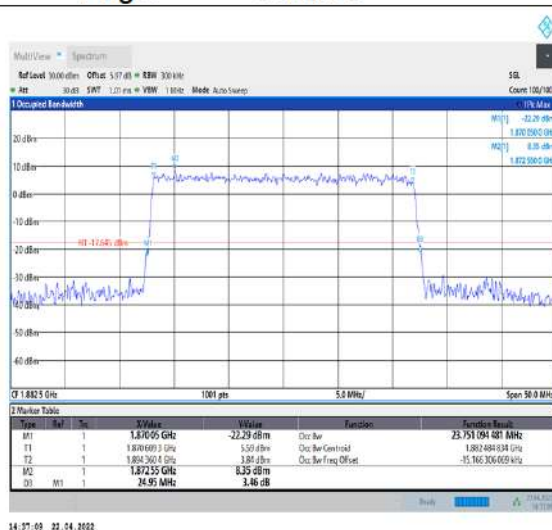
1-N25--15-25-M-9-CP-256QAM-Outet_Full-133@0-Ant1-23.751-24.950-≤25-PASS
