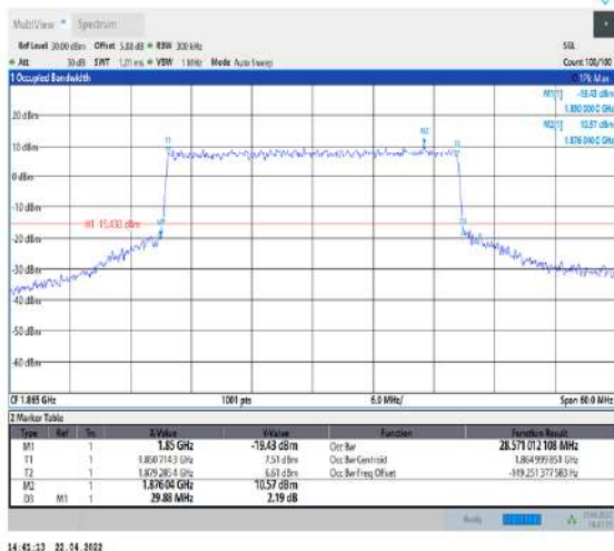
1-N25--15-30-L-8-CP-64QAM-Outer_Full-160@0-Ant1-28.571-29.880-≤30-PASS
