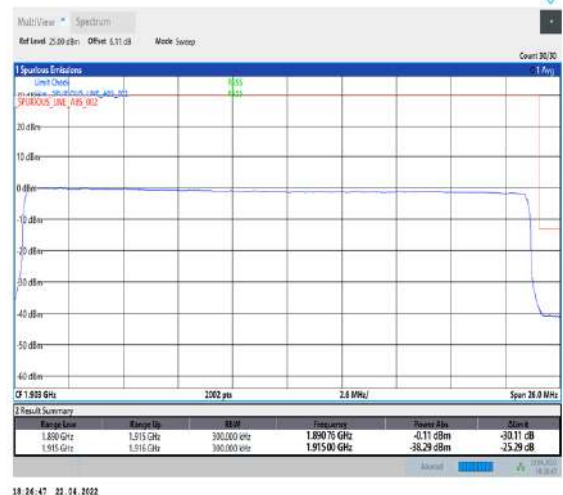
1-N25--15-25-H-6-CP-QPSK-Outer_Full-133@0-Ant1-seegraph-PASS-see graph
