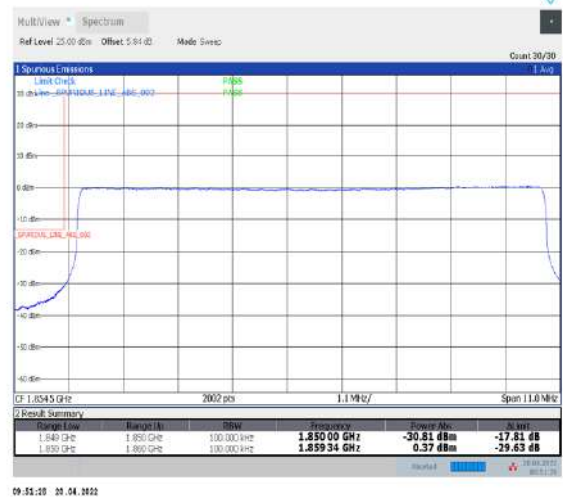
1-N25--15-10-L-6-CP-QPSK-Outer_Full-52@0-Ant1-seegraph-PASS-see graph
