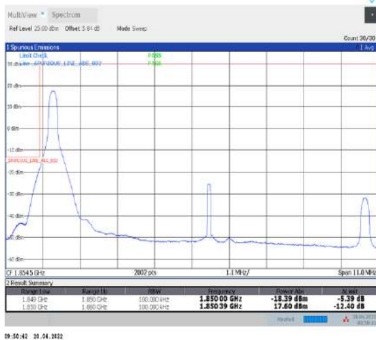
1-N25--15-10-L-4-CP-QPSK-Edge_1RB_Left-1@0-Ant1-seegraph-PASS-see graph
