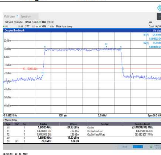
1-N25--15-25-L-6-CP-QPSK-Outer_Full-133@0-Ant1-23.782-25.100-≤25-PASS
