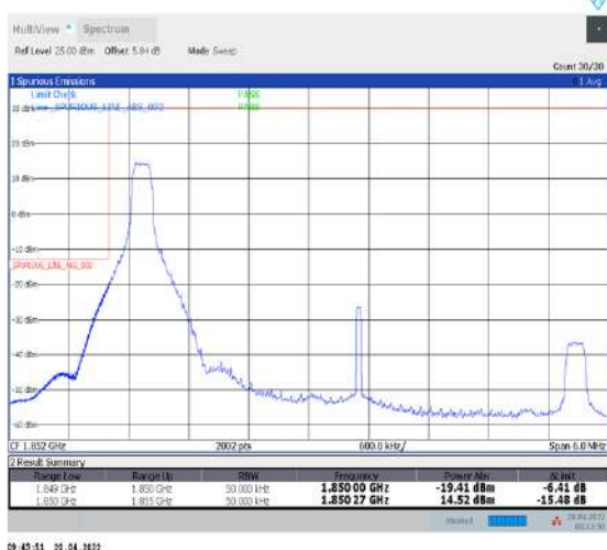
1-N25--15-5-L-4-CP-QPSK-Edge_1RB_Left-1@0-Ant1-seegraph-PASS-see graph
