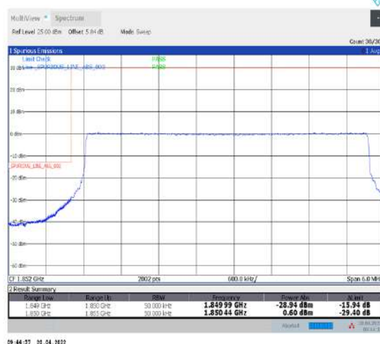
1-N25--15-5-L-6-CP-QPSK-Outer_Full-25@0-Ant1-seegraph-PASS-see graph
