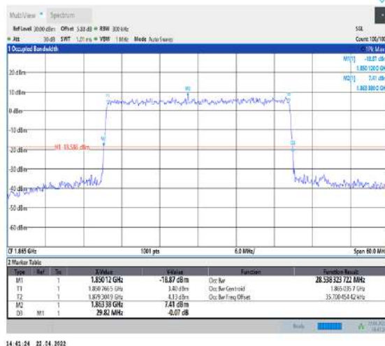
1-N25--15-30-L-9-CP-256QAM-Outer_Full-160@0-Ant1-28.538-29.820-≤30-PASS
