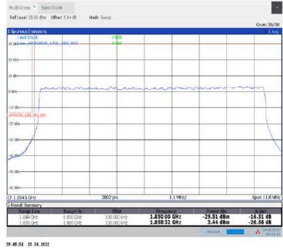
1-N25--15-10-L-3-DFT-PI2BPSK-Outer_Full-50@0-Ant1-seegraph-PASS-see graph
