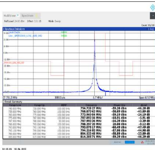
1-N14--15-5-L-1-DFT-PI2BPSK-Edge_1RB_Left-1@0-Ant1-PASS-see graph
