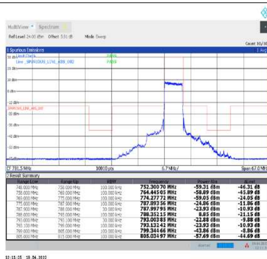
1-N14--15-5-L-3-DFT-PI2BPSK-Outer_Full-25@0-Ant1-PASS-see graph
