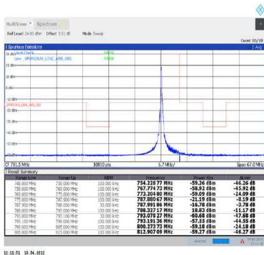
1-N14--15-5-L-4-CP-QPSK-Edge_1RB_Left-1@0-Ant1-PASS-see graph
