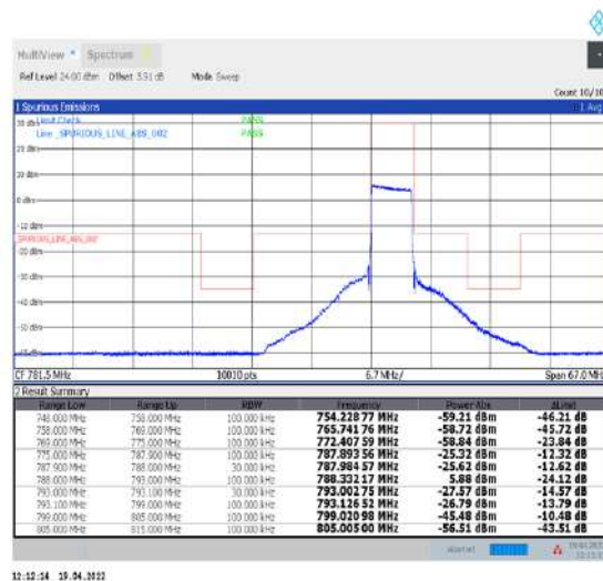
1-N14--15-5-L-6-CP-QPSK-Outer_Full-25@0-Ant1-PASS-see graph
