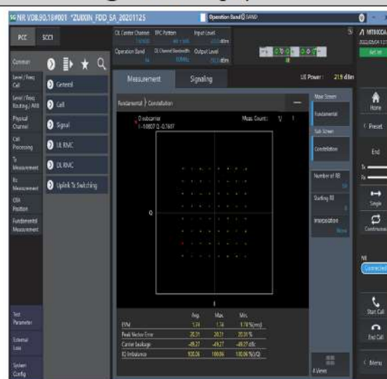
1-N14-PC3-15-10-M-4-DFT-64QAM-Outer_Full-50@0-Ant1-see graph-PASS
