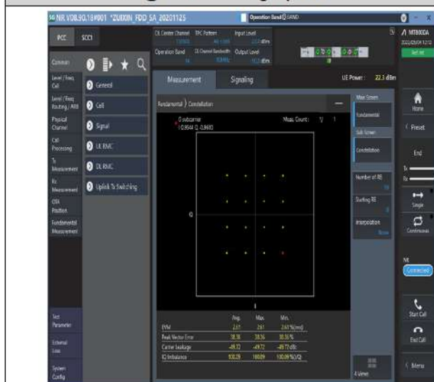
1-N14-PC3-15-10-M-3-DFT-16QAM-Outer_Full-50@0-Ant1-see graph-PASS
