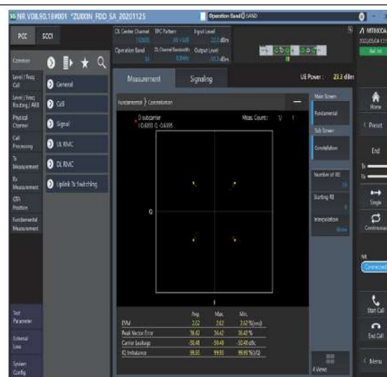
1-N14-PC3-15-10-M-2-DFT-QPSK-Outer_Full-50@0-Ant1-see graph-PASS
