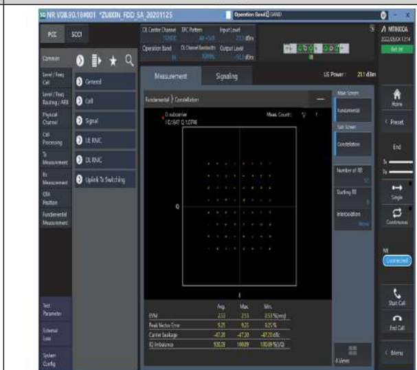
1-N14-PC3-15-10-M-8-CP-64QAM-Outer_Full-52@0-Ant1-see graph-PASS
