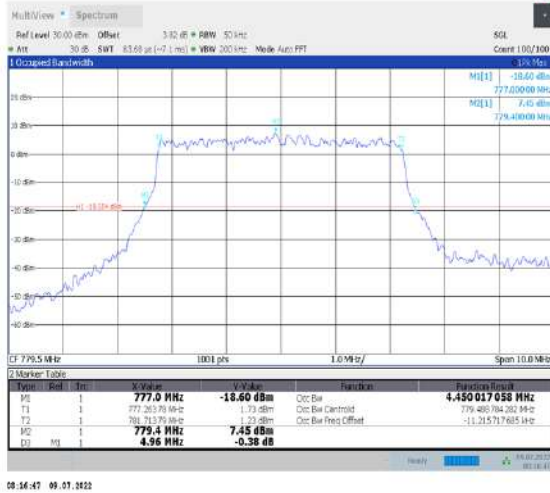
1-N13--15-5-L-9-CP-256QAM-Outer_Full-25@0-Ant1-4.45-4.960-≤5-PASS
