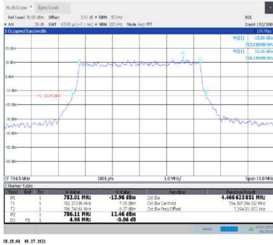
1-N13--15-5-H-3-DFT-16QAM-Outer_Full-25@0-Ant1-4.467-4.960-≤5-PASS
