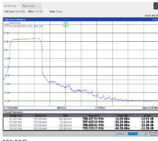
1-N13-PC3-15-5-H-3-DFT-PI2BPSK-Outer_Full-25@0-Ant1-PASS-see graph
