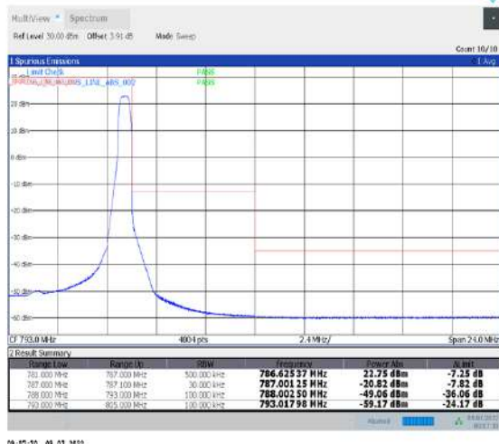
1-N13-PC3-15-5-H-2-DFT-PI2BPSK-Edge_1RB_Right-1@24-Ant1-PASS-see graph
