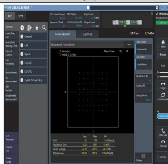
1-N13--15-10-M-4-DFT-64QAM-Outer_Full-50@0- Ant1-see graph-PASS
