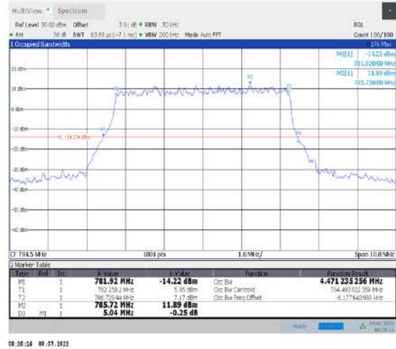
1-N13--15-5-H-4-DFT-64QAM-Outer_Full-25@0-Ant1-4.471-5.040-≤5-PASS
