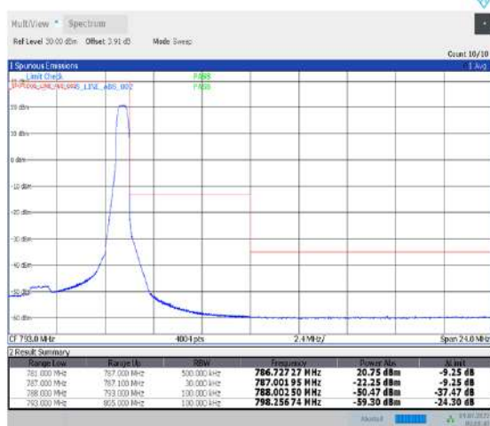
1-N13-PC3-15-5-H-5-CP-QPSK-Edge_1RB_Right-1@24-Ant1-PASS-see graph
