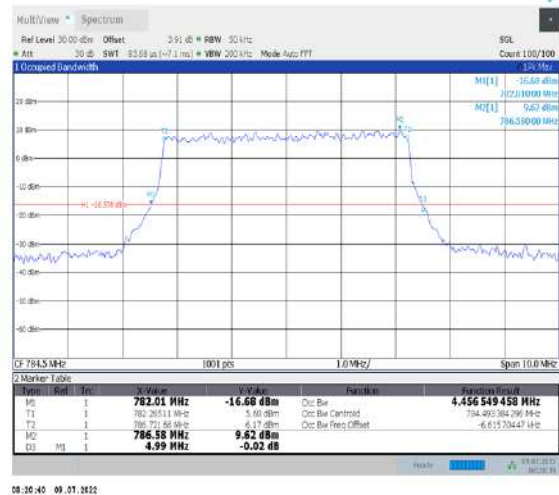
1-N13--15-5-H-6-CP-QPSK-Outer_Full-25@0-Ant1-4.457-4.990-≤5-PASS
