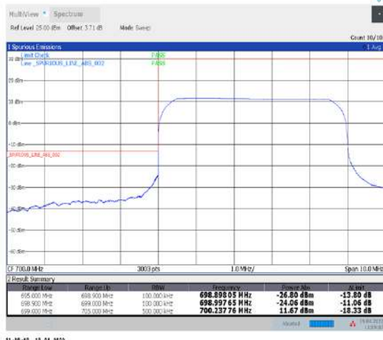
1-N12--15-5-L-6-CP-QPSK-Outer_Full-25@0-Ant1-PASS-see graph
