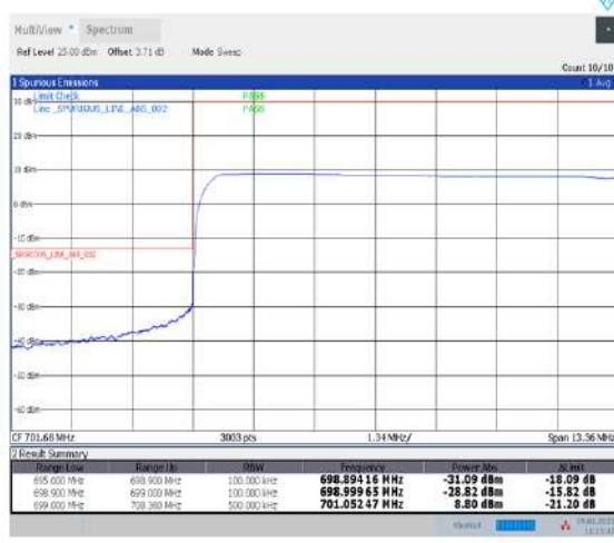
1-N12--15-10-L-6-CP-QPSK-Outer_Full-52@0-Ant1-PASS-see graph
