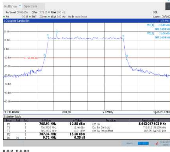
1-N12--15-10-H-1-DFT-QPSK-Outer_Full-50@0- Ant1-8.943-9.720-≤10-PASS
