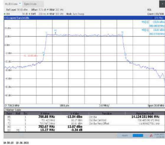
1-N12--15-15-H-6-CP-QPSK-Outer_Full-79@0-Ant1-13.45-14.610-≤15-PASS
