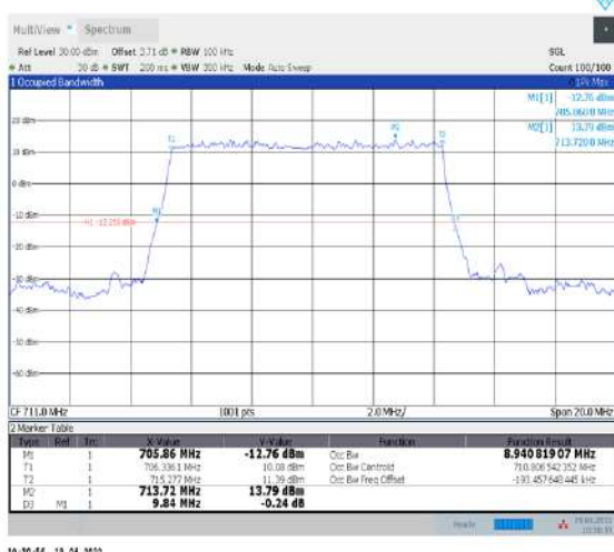
1-N12--15-10-H-2-DFT-PI2BPSK-Outer_Full-50@0- Ant1-8.941-9.840-≤10-PASS
