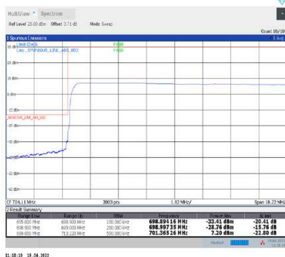
1-N12--15-15-L-6-CP-QPSK-Outer_Full-79@0-Ant1-PASS-see graph
