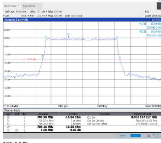
1-N12--15-10-H-5-DFT-256QAM-Outer_Full-50@0-Ant1-8.939-9.680-≤10-PASS
