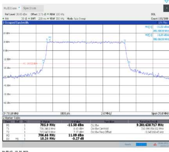
1-N12--15-10-H-6-CP-QPSK-Outer_Full-52@0-Ant1-9.302-10.240-≤10-PASS
