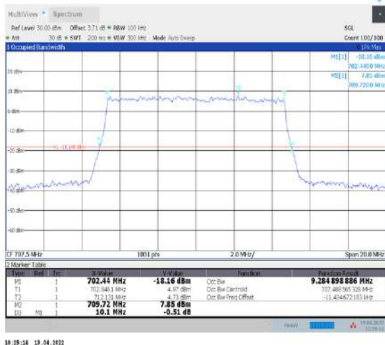
1-N12--15-10-M-9-CP-256QAM-Outer_Full-52@0- Ant1-9.285-10.100-≤10-PASS
