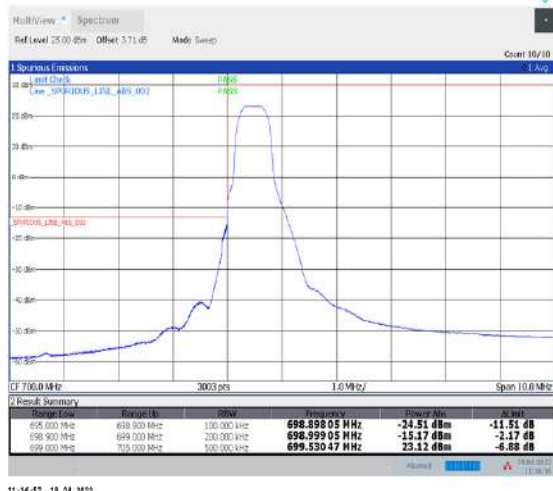
1-N12--15-15-L-1-DFT-PI2BPSK-Edge_1RB_Left-1@0-Ant1-PASS-see graph
