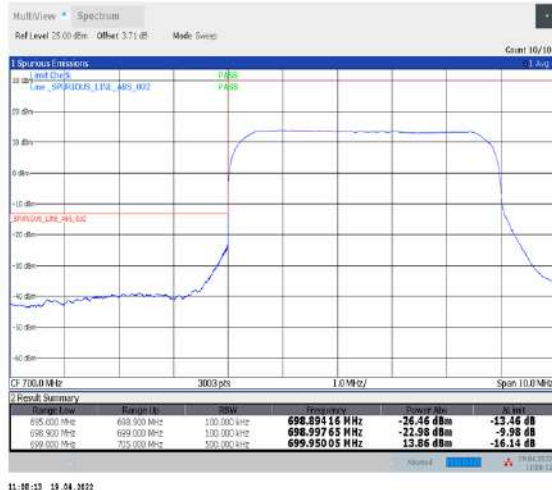
1-N12--15-5-L-3-DFT-PI2BPSK-Outer_Full-25@0-Ant1-PASS-see graph
