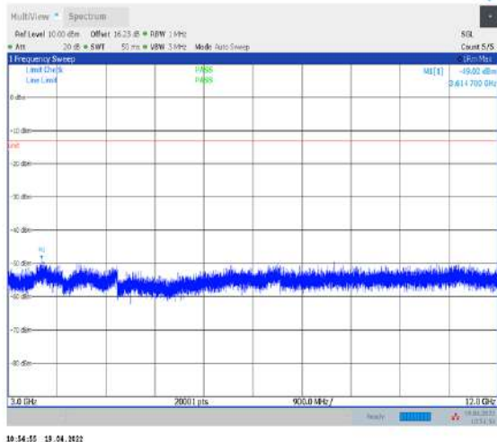
1-N12--15-15-H-1-DFT-PI2BPSK-Inner_1RB_Left- 1@1-3000-12000-Ant1--49.02--13-PASS
