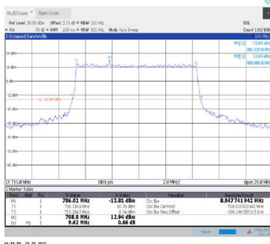
1-N12--15-10-H-3-DFT-16QAM-Outer_Full-50@0- Ant1-8.948-9.620-≤10-PASS
