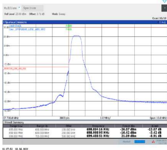
1-N12--15-15-L-4-CP-QPSK-Edge_1RB_Left-1@0-Ant1-PASS-see graph
