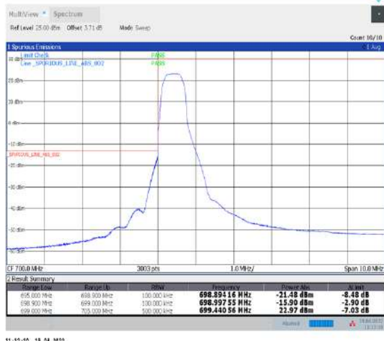
1-N12--15-10-L-1-DFT-PI2BPSK-Edge_1RB_Left-1@0-Ant1-PASS-see graph
