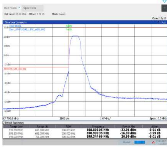
1-N12--15-10-L-4-CP-QPSK-Edge_1RB_Left-1@0-Ant1-PASS-see graph
