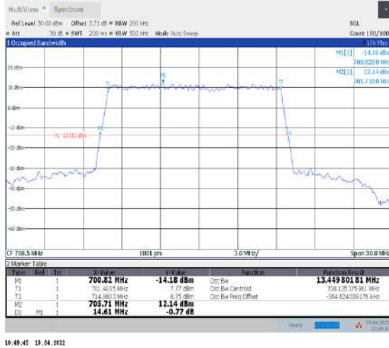
1-N12--15-15-H-5-DFT-256QAM-Outer_Full-75@0-Ant1-13.45-14.610-≤15-PASS
