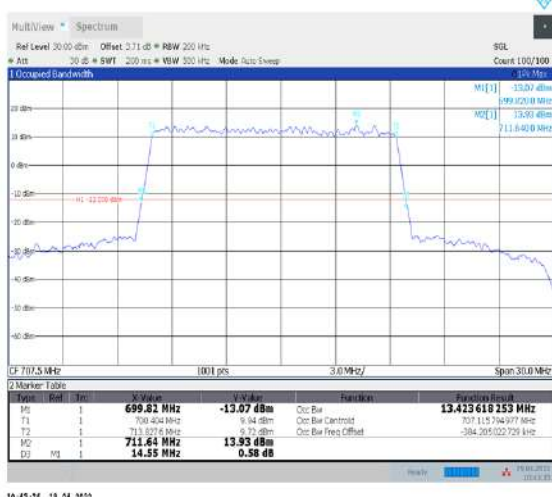
1-N12--15-15-M-4-DFT-64QAM-Outer_Full-75@0-Ant1-13.424-14.550-≤15-PASS
