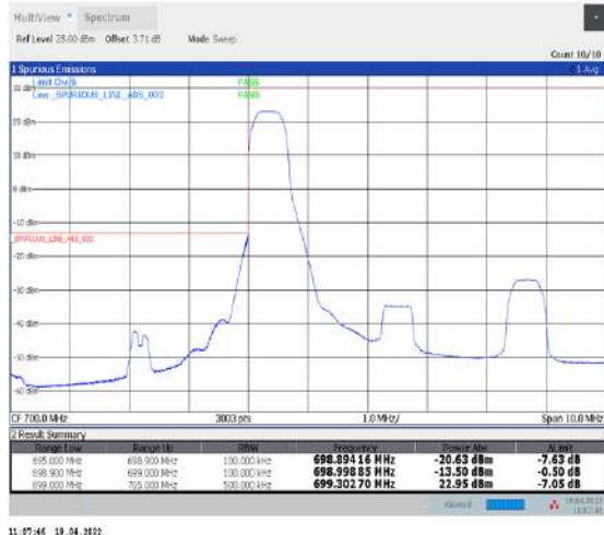
1-N12--15-5-L-1-DFT-PI2BPSK-Edge_1RB_Left-1@0-Ant1-PASS-see graph
