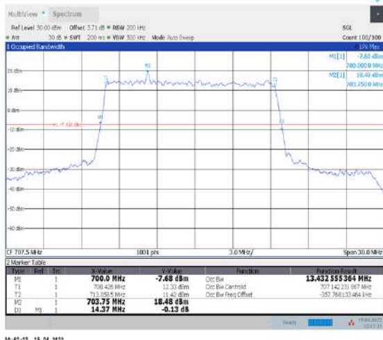
1-N12--15-15-M-2-DFT-PI2BPSK-Outer_Full-75@0-Ant1-13.433-14.370-≤15-PASS
