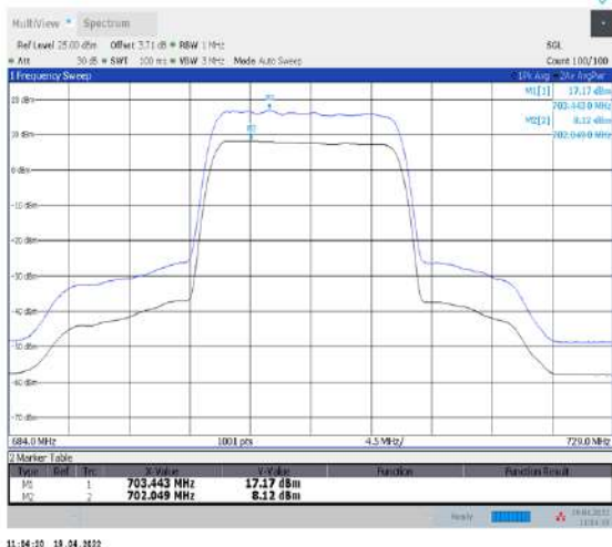
1-N12--15-15-L-1-DFT-256QAM-Outer_Full-75@0- Ant1-9.05-100%-0.00-9.05-PASS-≤13
