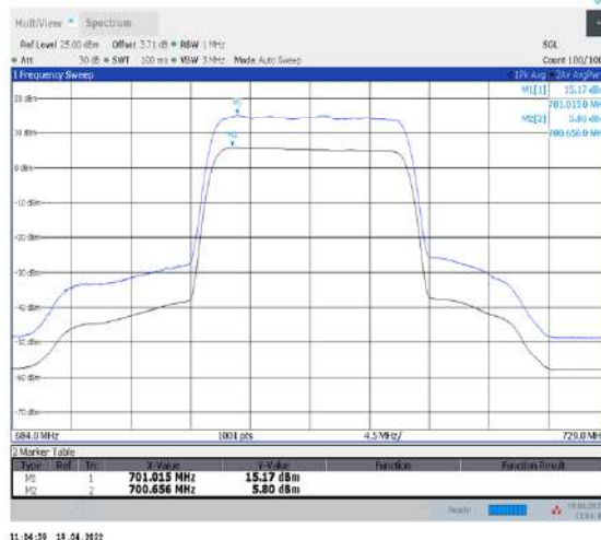
1-N12--15-15-L-2-CP-256QAM-Outer_Full-79@0- Ant1-9.37-100%-0.00-9.37-PASS-≤13
