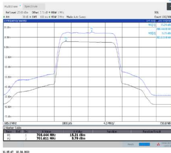
1-N12--15-15-M-2-CP-256QAM-Outer_Full-79@0- Ant1-9.42-100%-0.00-9.42-PASS-≤13
