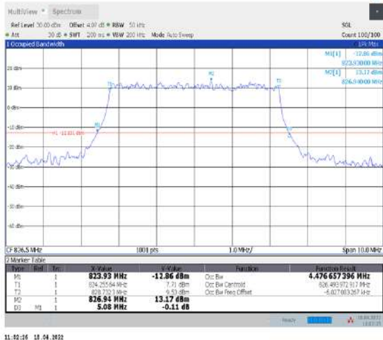
1-N5--15-5-L-3-DFT-16QAM-Outer_Full-25@0-Ant1-4.477-5.080-≤5-PASS
