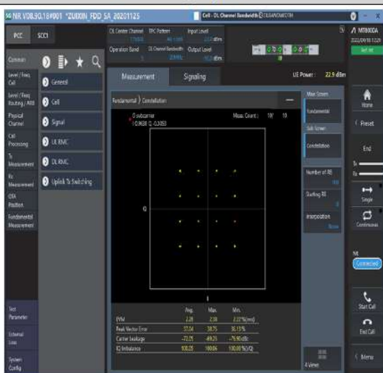
1-N5--15-20-M-3-DFT-16QAM-Outer_Full-100@0-Ant1-see graph-PASS
