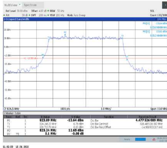
1-N5--15-5-L-4-DFT-64QAM-Outer_Full-25@0-Ant1-4.478-5.100-≤5-PASS
