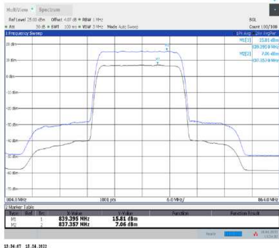
1-N5--15-20-L-1-DFT-256QAM-Outer_Full-100@0- Ant1-8.75-100%-0.00-8.75-PASS-≤13
