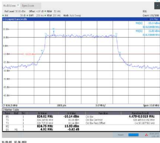
1-N5--15-5-L-1-DFT-QPSK-Outer_Full-25@0-Ant1-4.479-4.920-≤5-PASS
