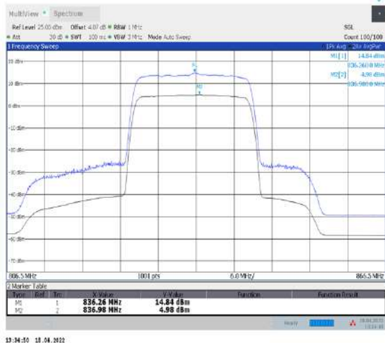
1-N5--15-20-M-1-DFT-256QAM-Outer_Full-100@0- Ant1-9.86-100%-0.00-9.86-PASS-≤13
