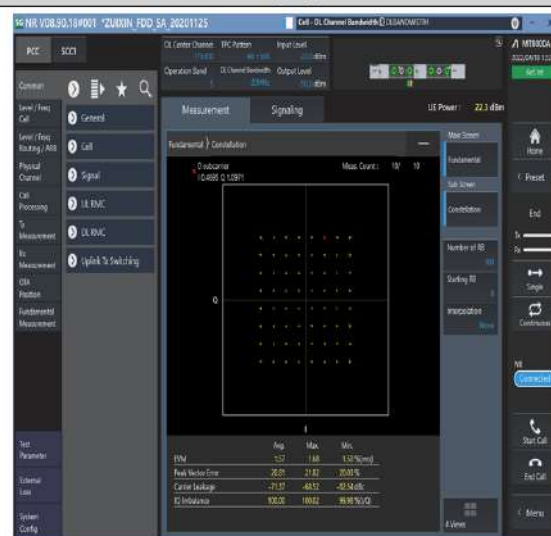
1-N5--15-20-M-4-DFT-64QAM-Outer_Full-100@0-Ant1-see graph-PASS
