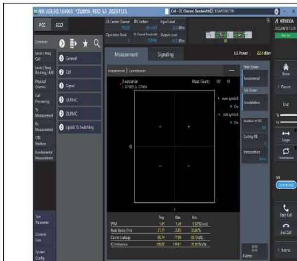
1-N5--15-20-M-1-DFT-PI2BPSK-Outer_Full-100@0-Ant1-see graph-PASS
