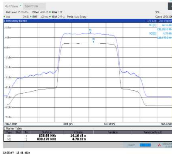
1-N5--15-20-M-2-CP-256QAM-Outer_Full-106@0- Ant1-9.46-100%-0.00-9.46-PASS-≤13
