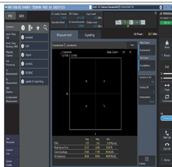
1-N5--15-20-M-2-DFT-QPSK-Outer_Full-100@0-Ant1-see graph-PASS
