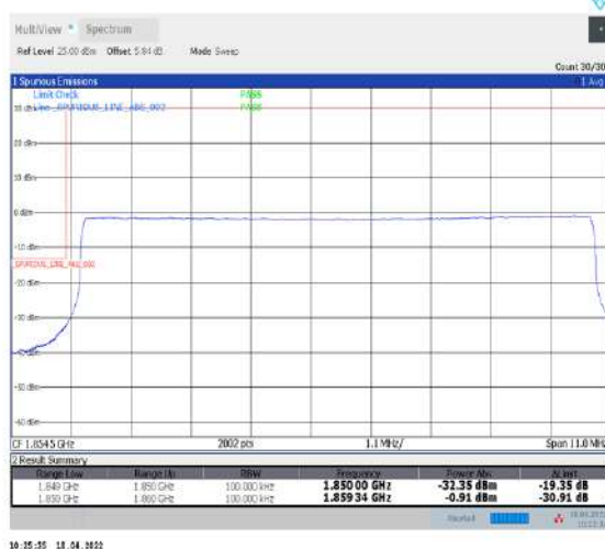
1-N2--15-10-L-6-CP-QPSK-Outer_Full-52@0-Ant1-seegraph-PASS-see graph
