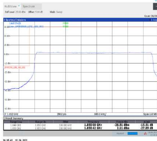
1-N2--15-5-L-6-CP-QPSK-Outer_Full-25@0-Ant1-seegraph-PASS-see graph
