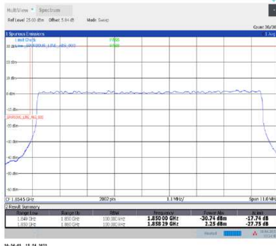
1-N2--15-10-L-3-DFT-PI2BPSK-Outer_Full-50@0-Ant1-seegraph-PASS-see graph
