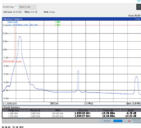
1-N2--15-10-L-4-CP-QPSK-Edge_1RB_Left-1@0-Ant1-seegraph-PASS-see graph
