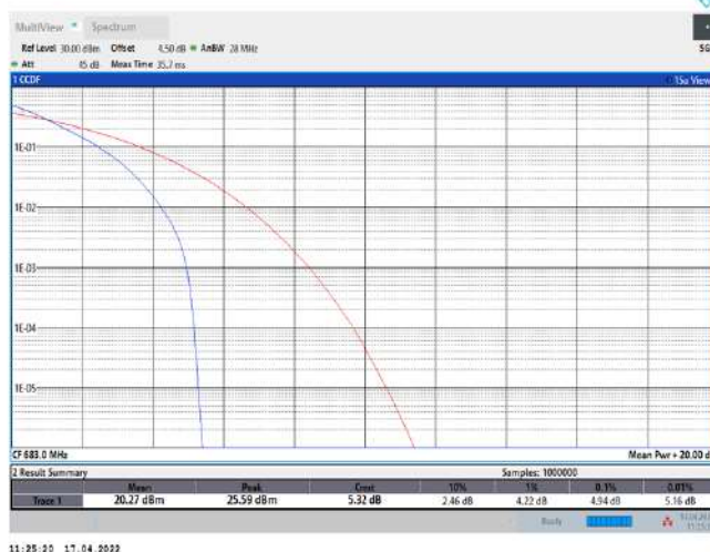
Band71-20MHz-QPSK-133322-100RB#0
