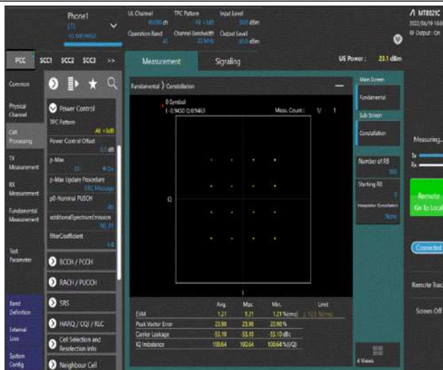
Band43-20MHz-16QAM-45090-100RB#0
