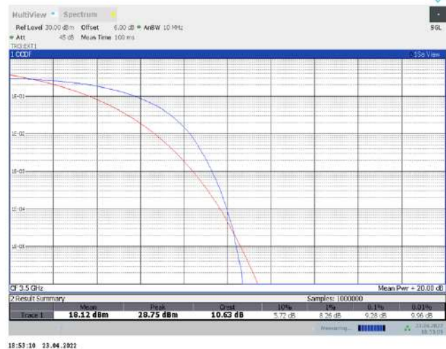
Band42-20MHz-QPSK-42590-100RB#0
