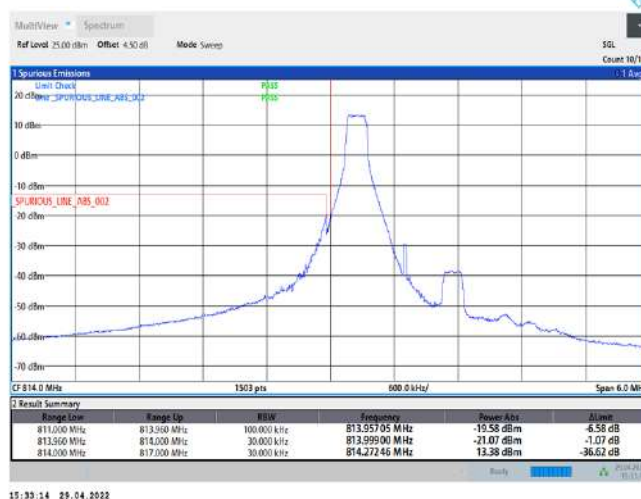
Band26-1.4MHz-QPSK-26697-6RB#0
