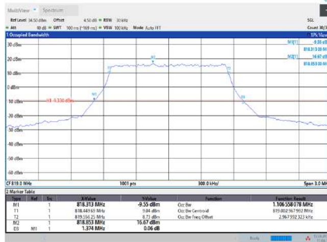
Band26-1.4MHz-QPSK-26740-6RB#0
