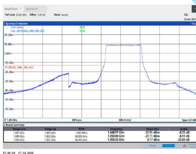
Band25-1.4MHz-QPSK-26047-6RB#0
