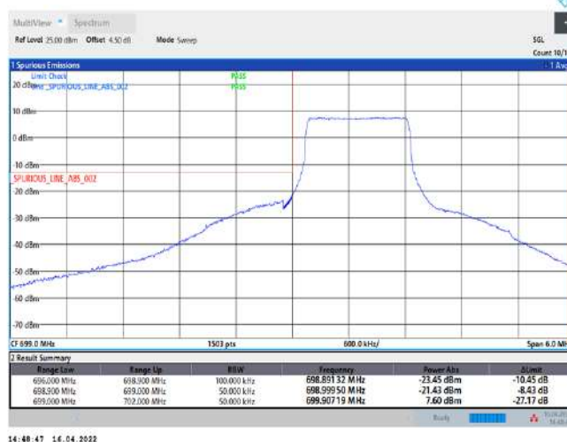
Band12-1.4MHz-QPSK-23017-6RB#0
