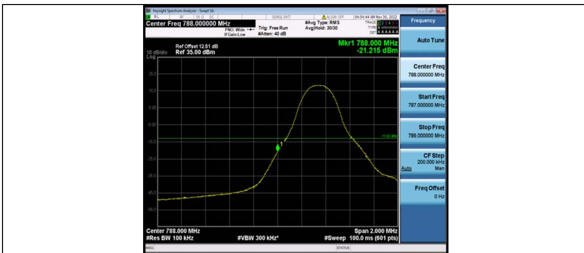
Band14-5MHz-64QAM-23305-25RB#0
