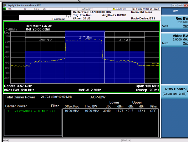
N48-40MHz-QPSK-641666-1RB#0
