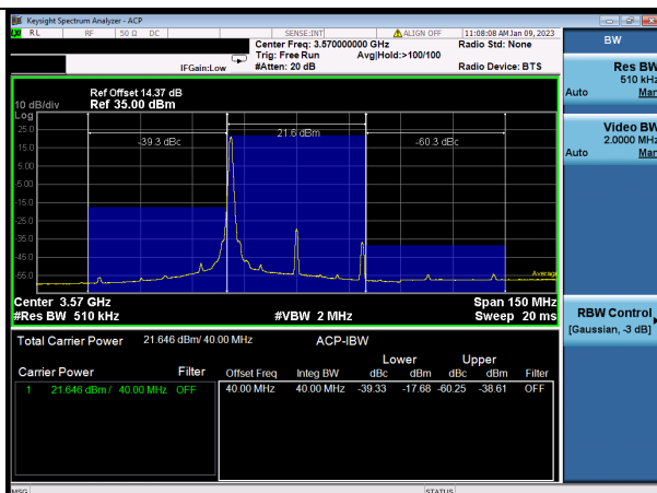
N48-40MHz-QPSK-638000-1RB#104
