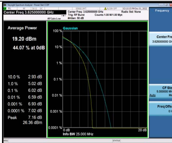
Band48-20MHz-16QAM-56640-1RB#0
