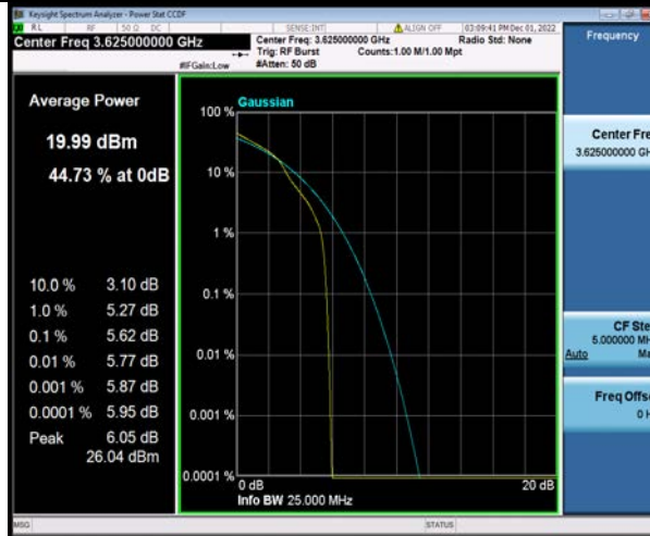
Band48-20MHz-16QAM-55990-100RB#0
