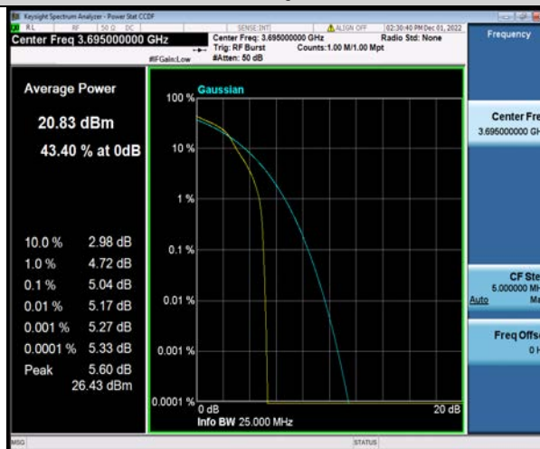
Band48-10MHz-16QAM-56690-50RB#0
