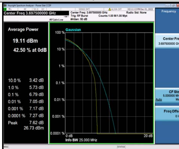
Band48-5MHz-64QAM-56715-25RB#0
