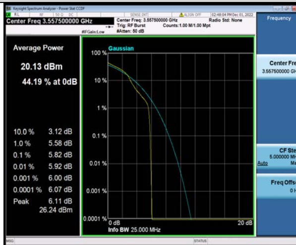
Band48-15MHz-16QAM-55315-75RB#0
