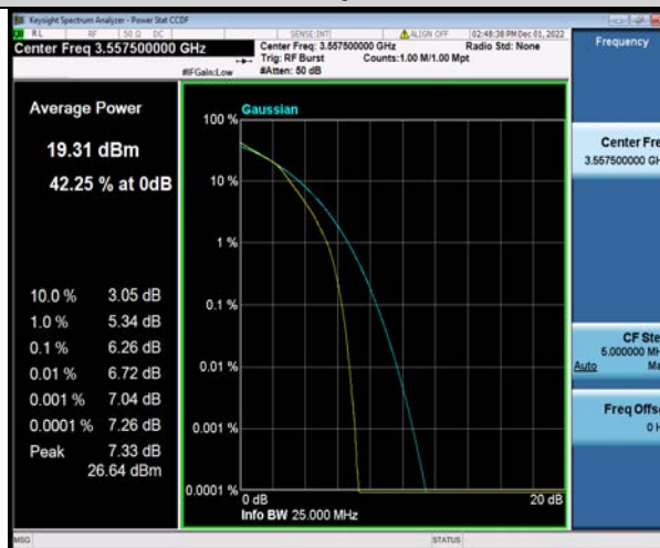
Band48-15MHz-16QAM-55990-1RB#0
