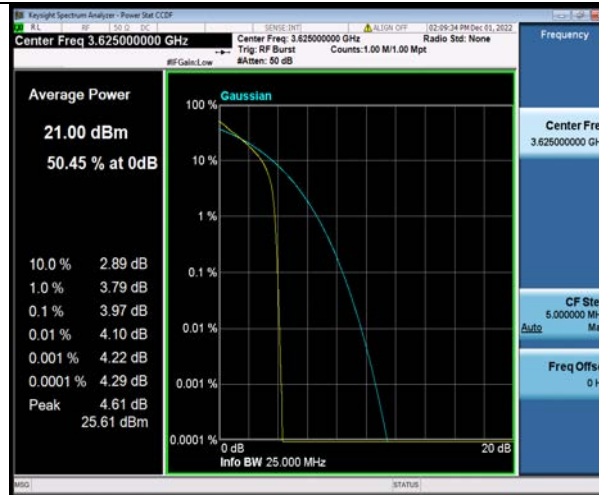
Band48-5MHz-QPSK-55990-25RB#0
