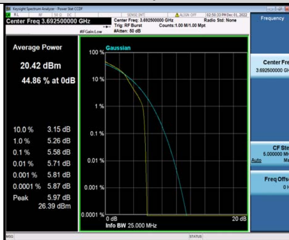
Band48-15MHz-16QAM-56665-75RB#0
