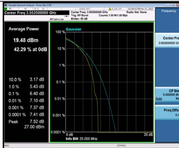
Band48-5MHz-64QAM-55265-25RB#0
