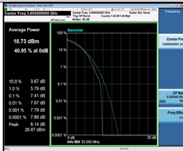
Band48-10MHz-64QAM-56690-50RB#0
