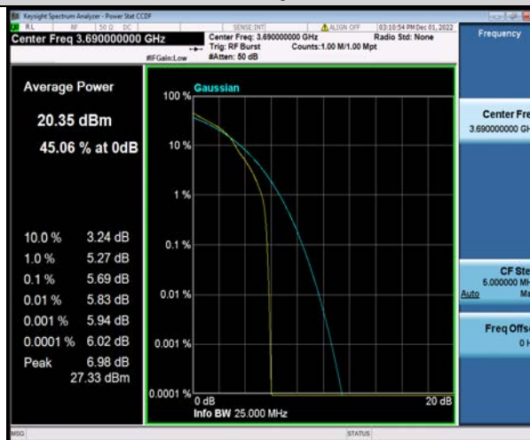
Band48-20MHz-16QAM-56640-100RB#0
