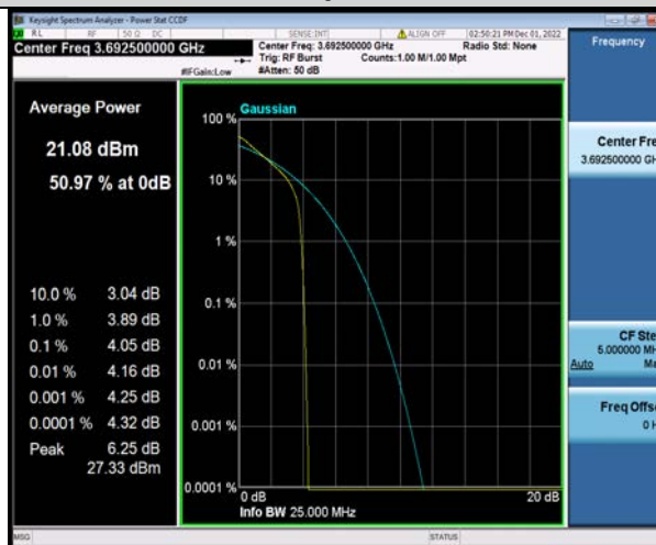
Band48-15MHz-QPSK-56665-75RB#0
