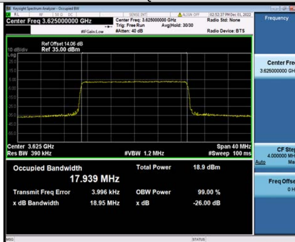
Band48-20MHz-64QAM-56640-100RB#0
