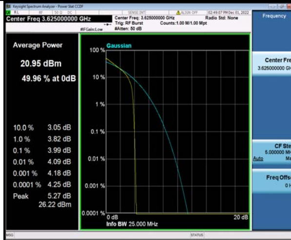
Band48-15MHz-QPSK-55990-75RB#0
