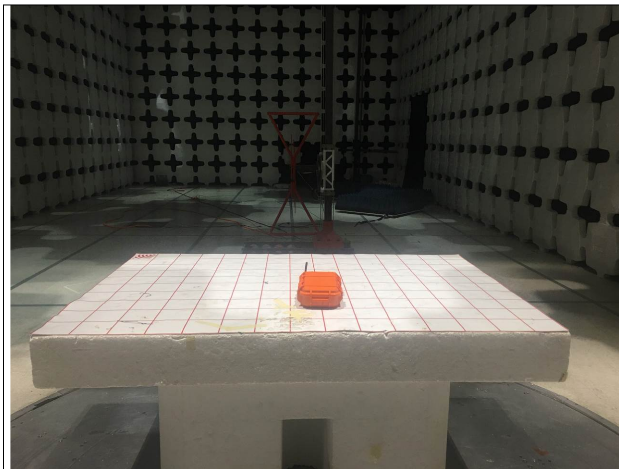
Radiated Emission Test below 1GHz Rear View
