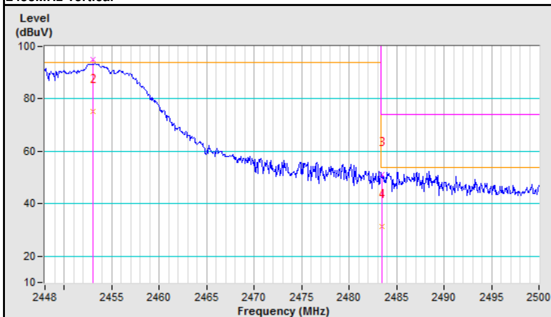
2453MHz Vertical
