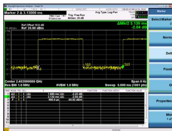
Modulation Mode: \pi/4 -DQPSK (DH3)
