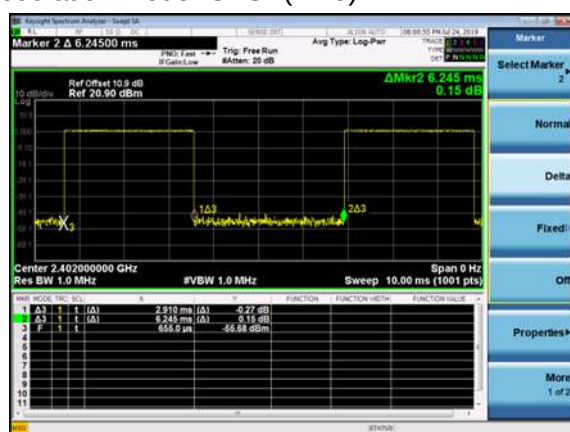
Modulation Mode: GFSK(DH5)
