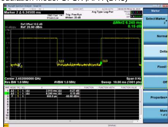
Modulation Mode: GFSK ,AFH (DH5)
