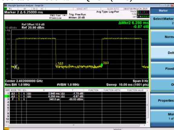
Modulation Mode: \pi/4 -DQPSK (DH5)
