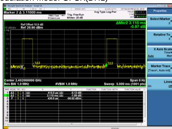
Modulation Mode: GFSK(DH1)
