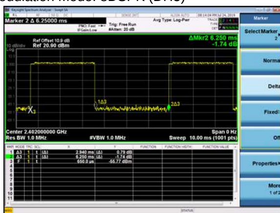
Modulation Mode: 8DSPK (DH5)
