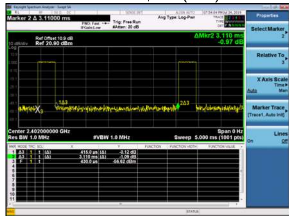
Modulation Mode: GFSK ,AFH (DH1)
