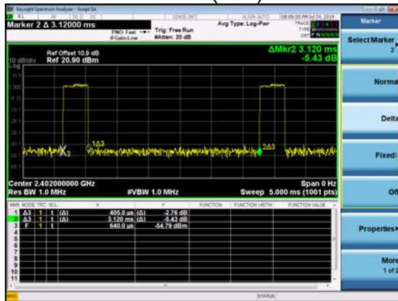
Modulation Mode: 8DSPK (DH1)
