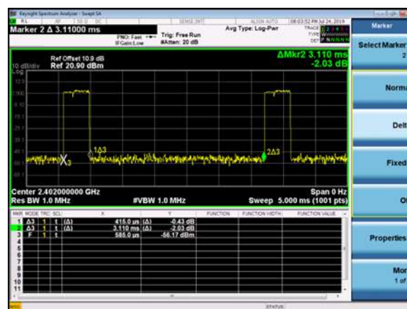
Modulation Mode: \pi/4 -DQPSK (DH1)
