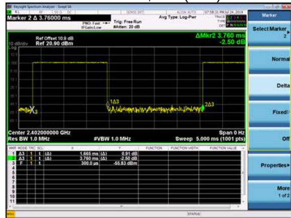
Modulation Mode: GFSK ,AFH (DH3)
