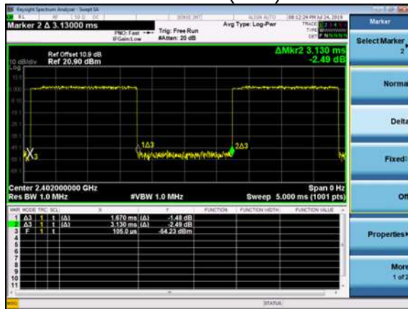
Modulation Mode: 8DSPK (DH3)
