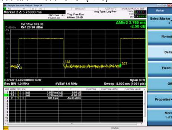
Modulation Mode: GFSK(DH3)
