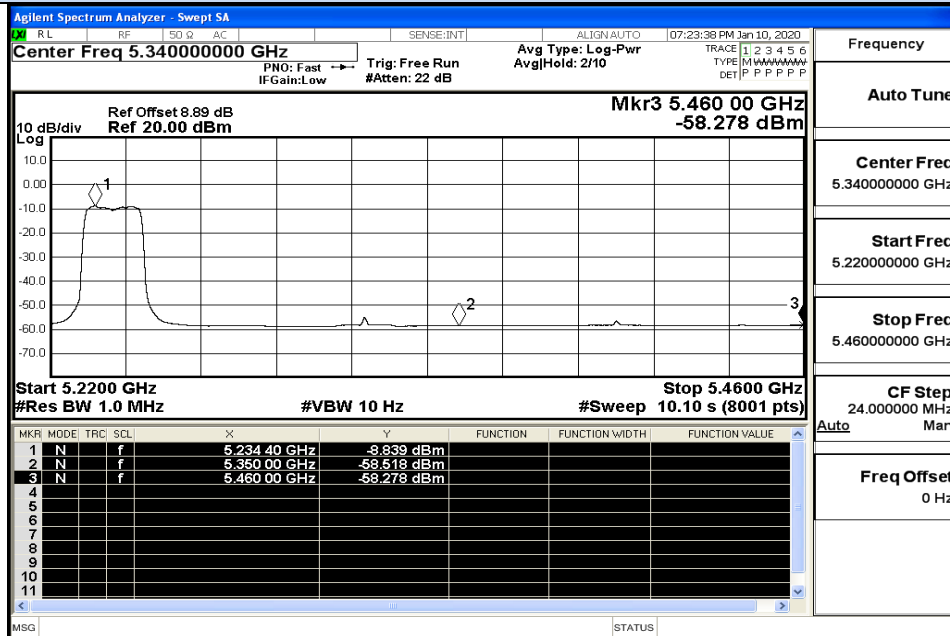
IEEE 802.11ac20 / Channel 48 / 5240MHz / Average
