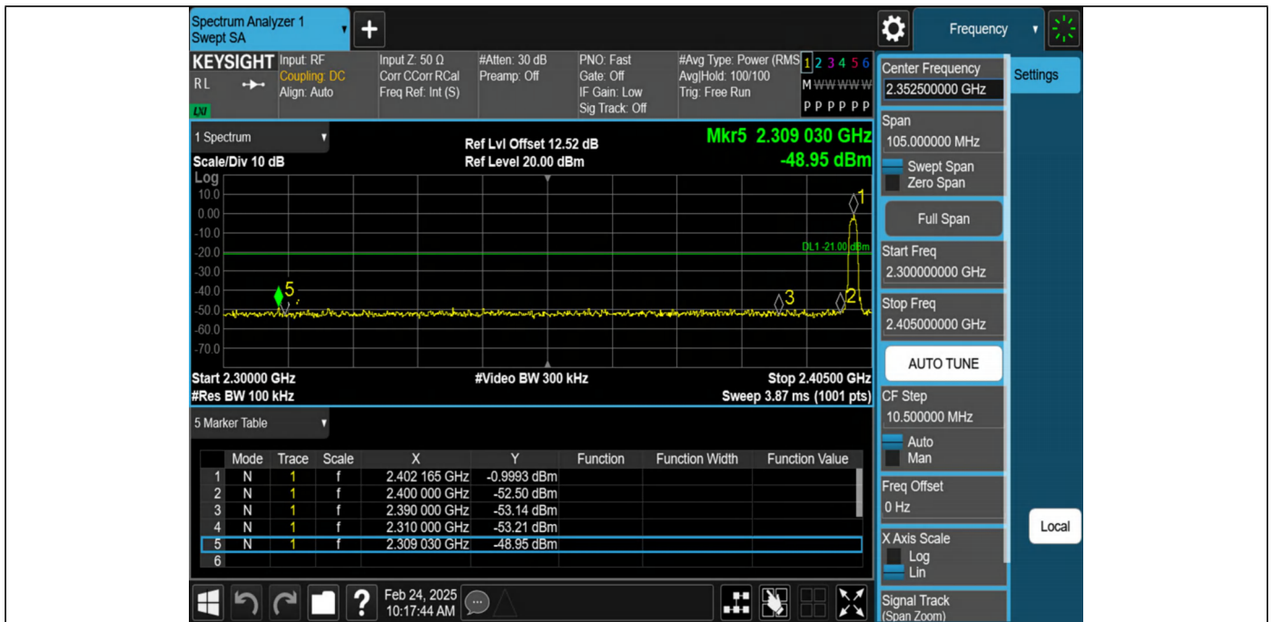
2DH5-Ant1-2402-PASS
