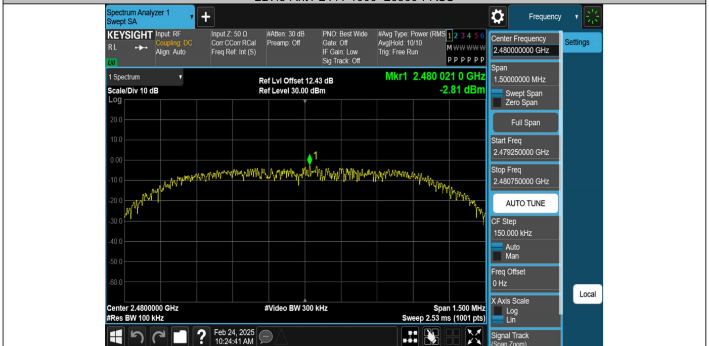
2DH5-Ant1-2480-0~Reference-PASS
