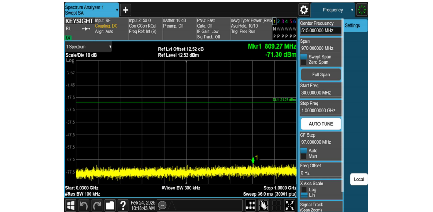
2DH5-Ant1-2402-30~1000-PASS
