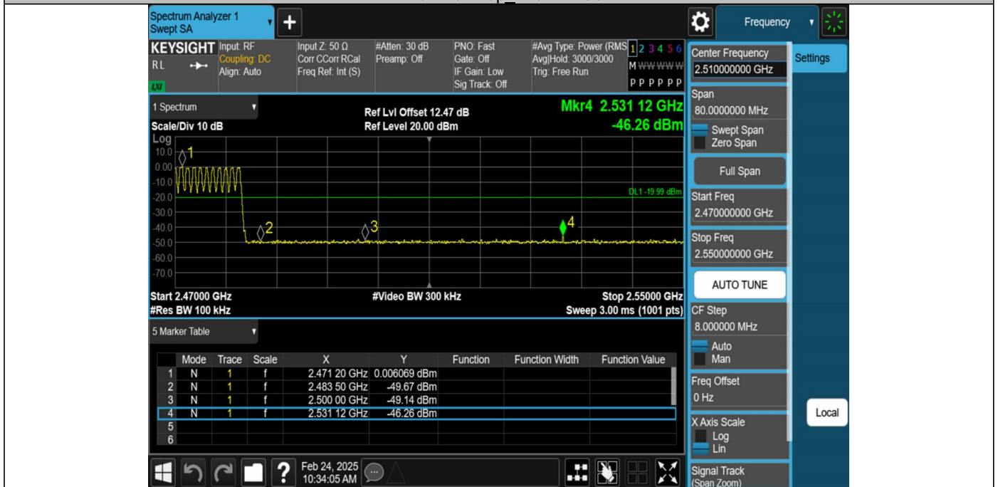
DH5-Ant1-Hop_2480-PASS
