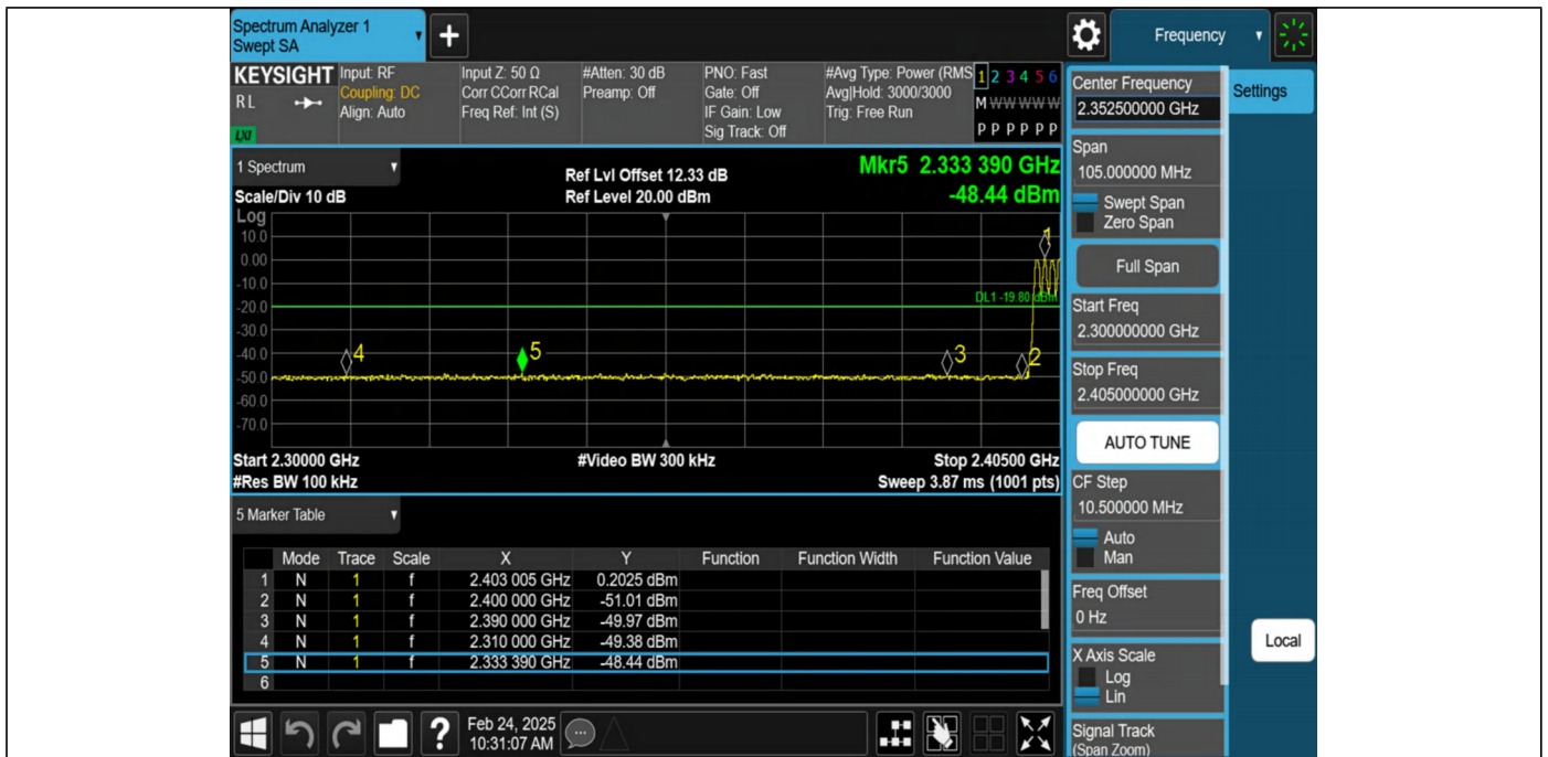
DH5-Ant1-Hop_2402-PASS
