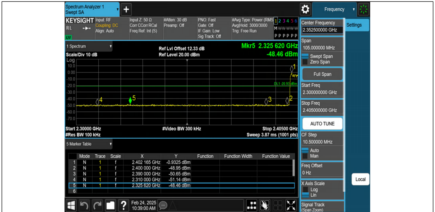
2DH5-Ant1-Hop_2402-PASS
