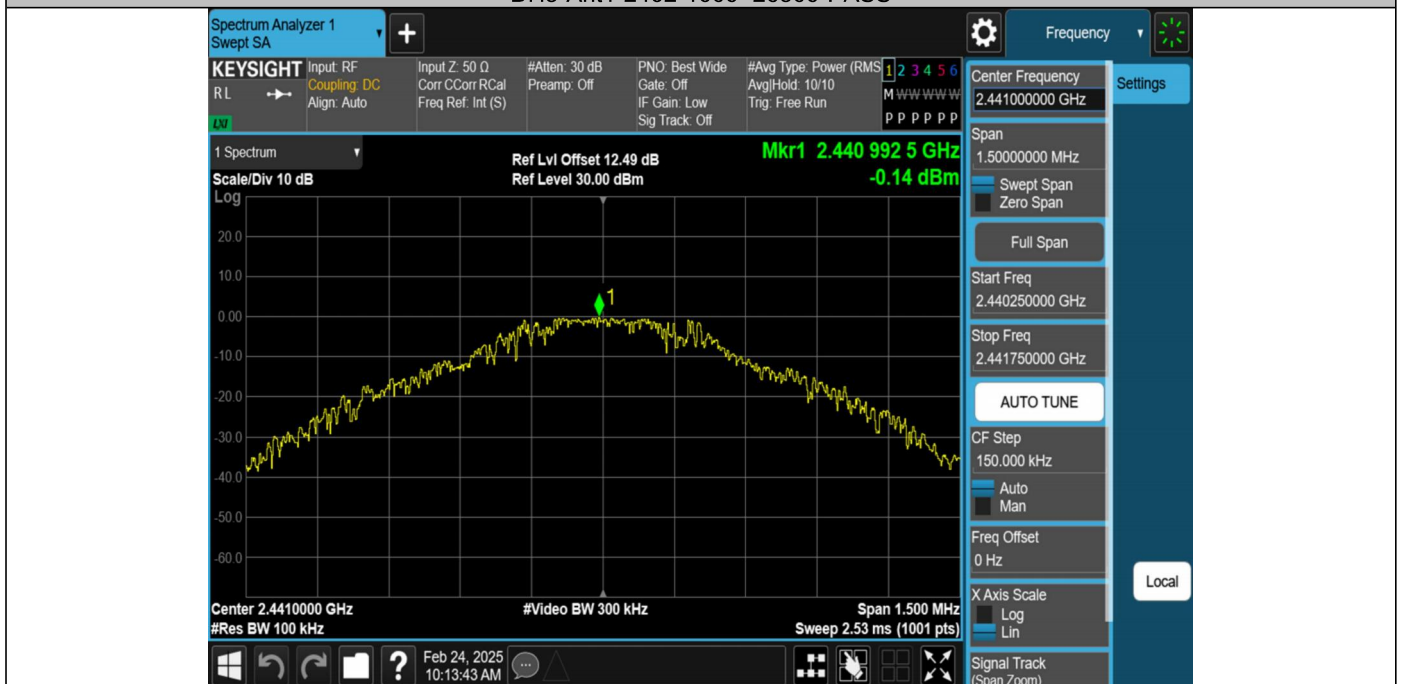
DH5-Ant1-2441-0~Reference-PASS
