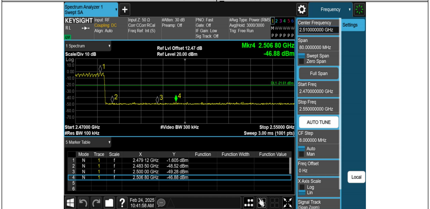
2DH5-Ant1-Hop_2480-PASS
