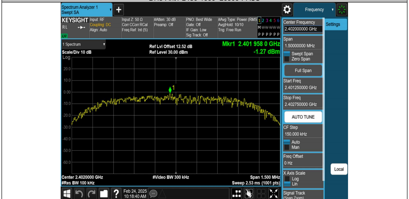
2DH5-Ant1-2402-0~Reference-PASS
