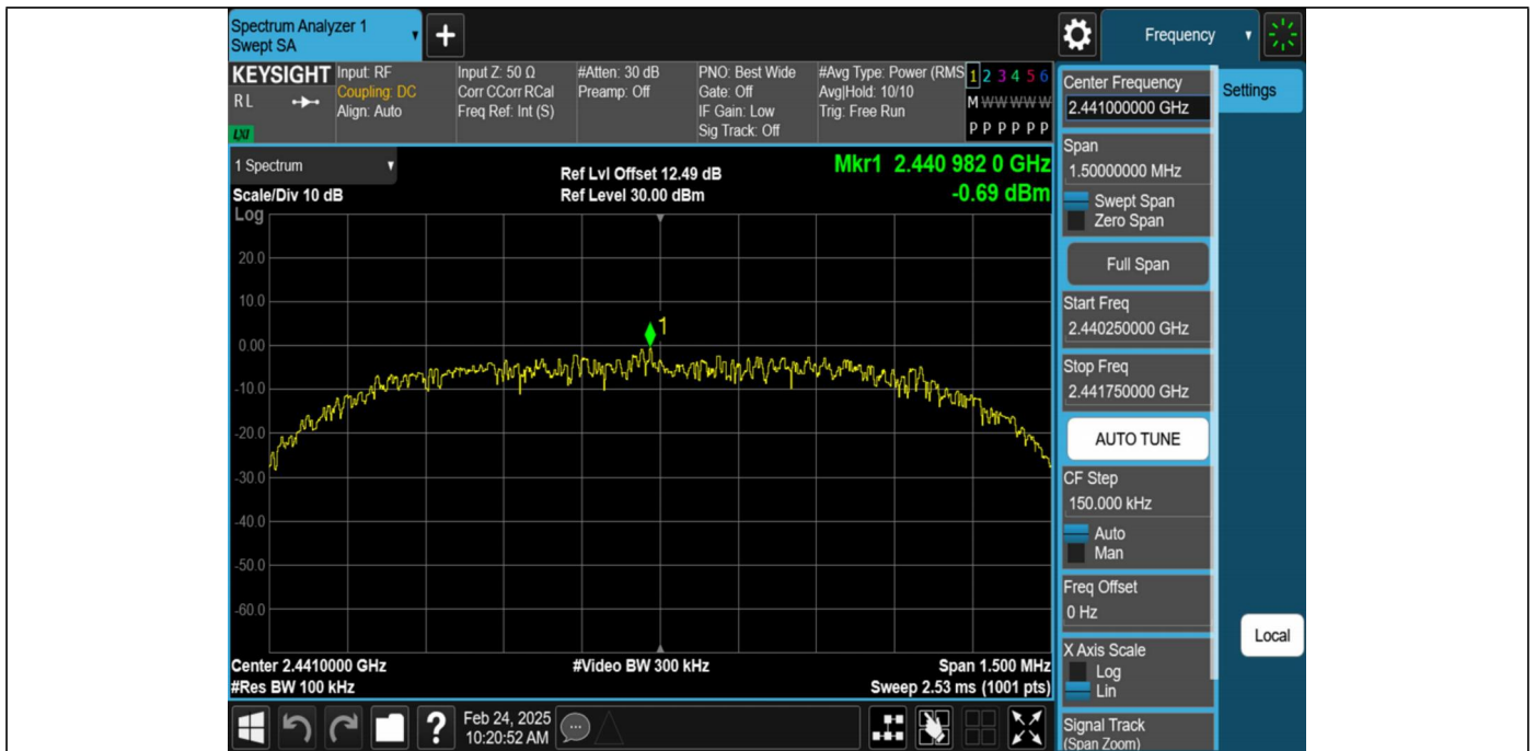
2DH5-Ant1-2441-0~Reference-PASS
