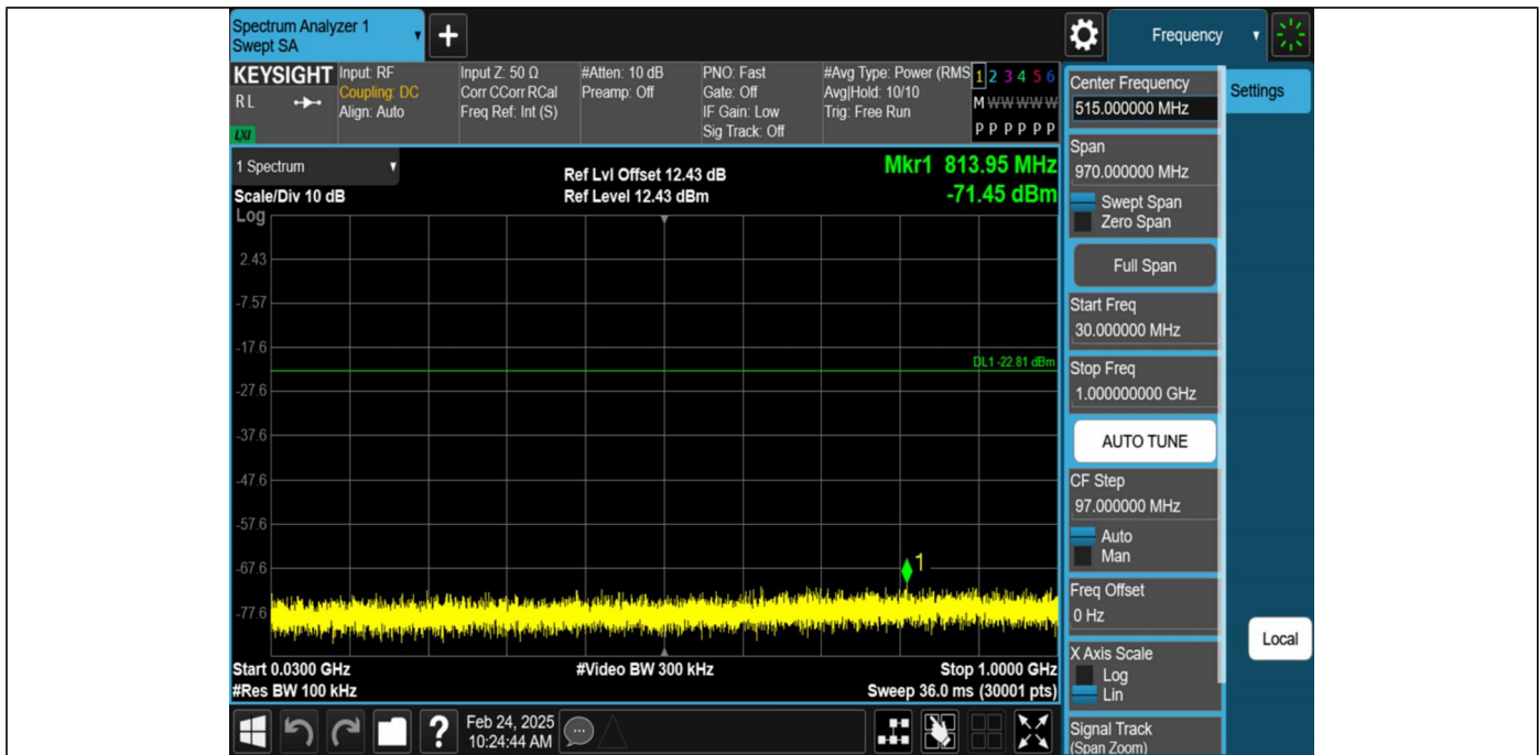
2DH5-Ant1-2480-30~1000-PASS
