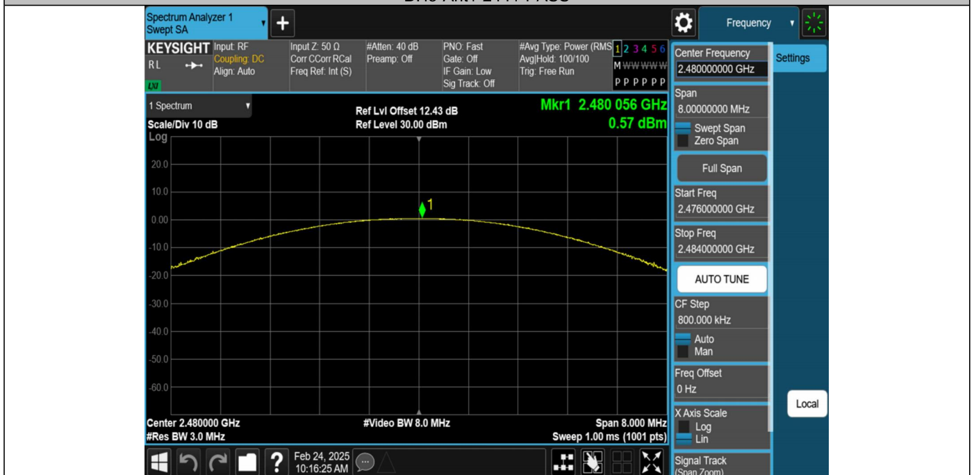
DH5-Ant1-2480-PASS
