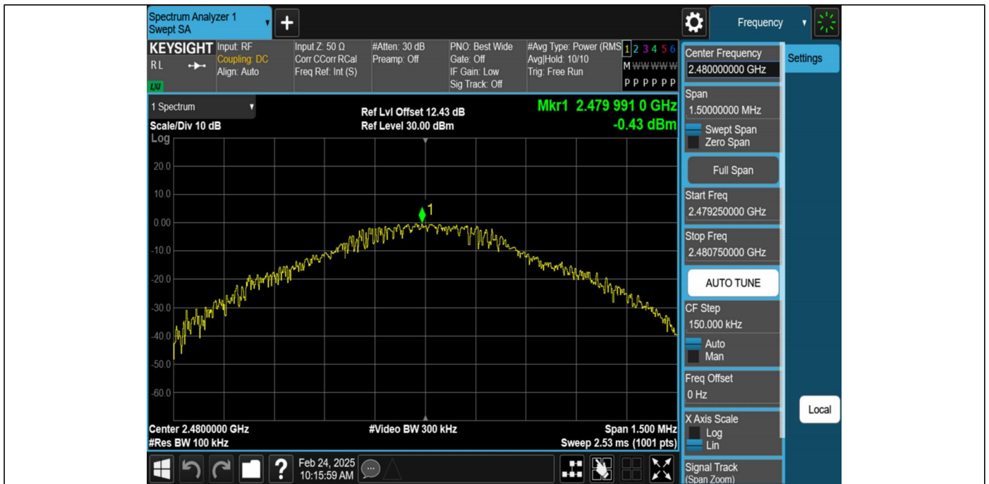
DH5-Ant1-2480-0~Reference-PASS
