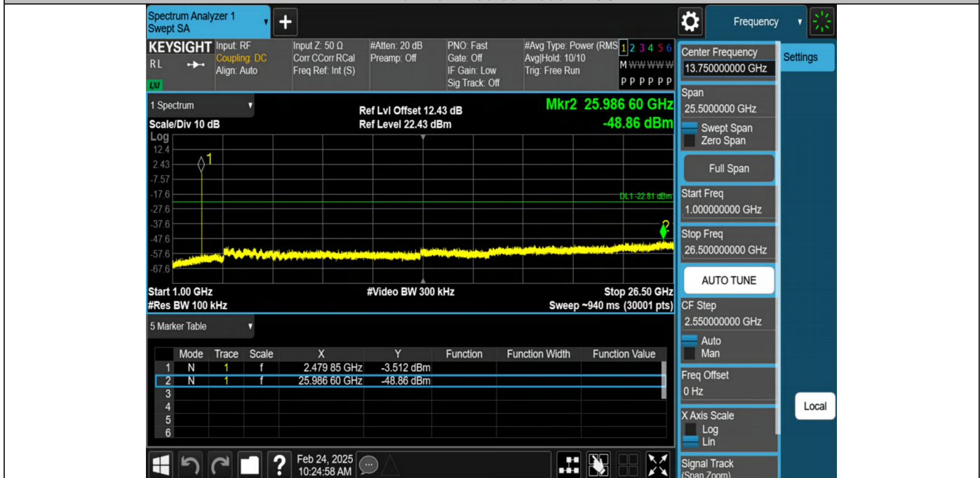
2DH5-Ant1-2480-1000~26500-PASS
