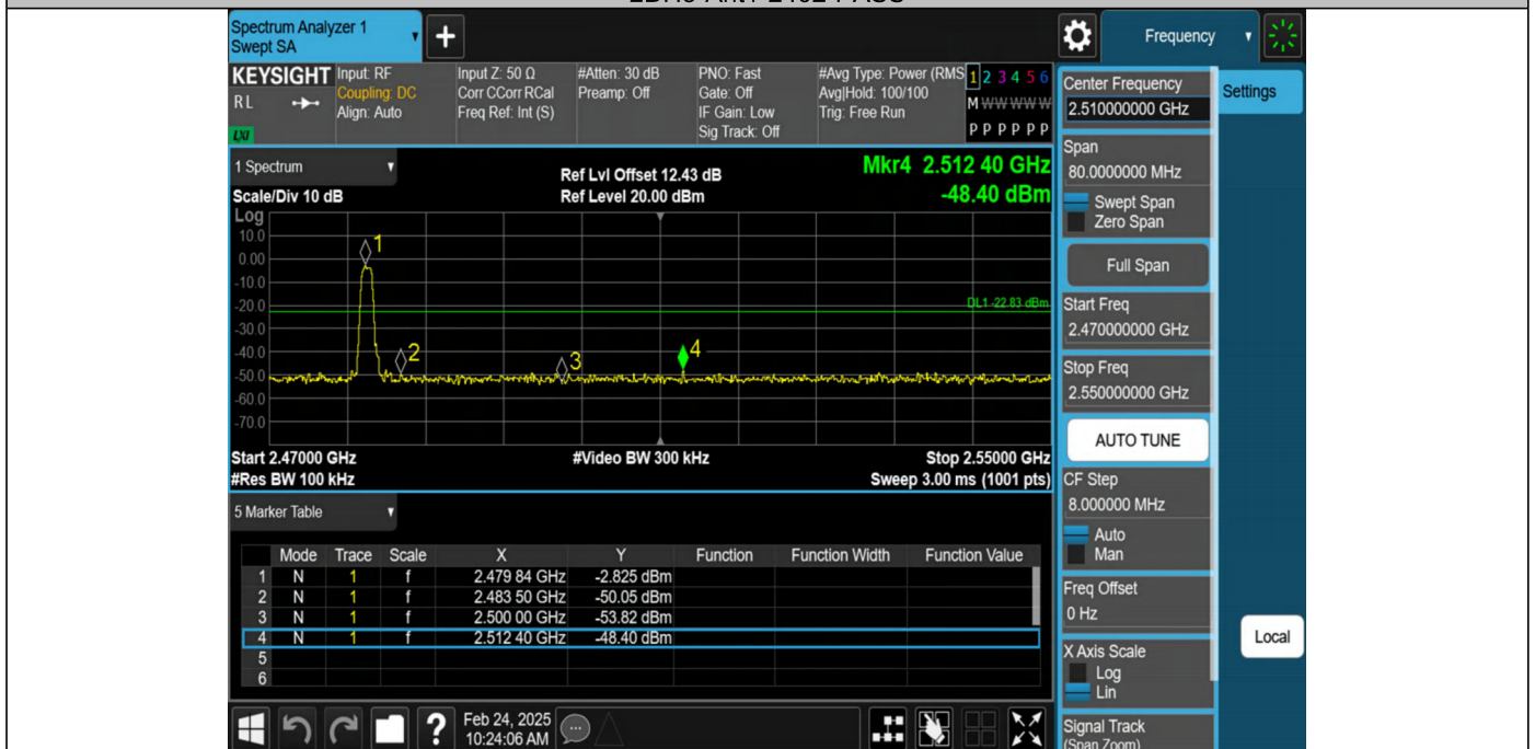
2DH5-Ant1-2480-PASS
