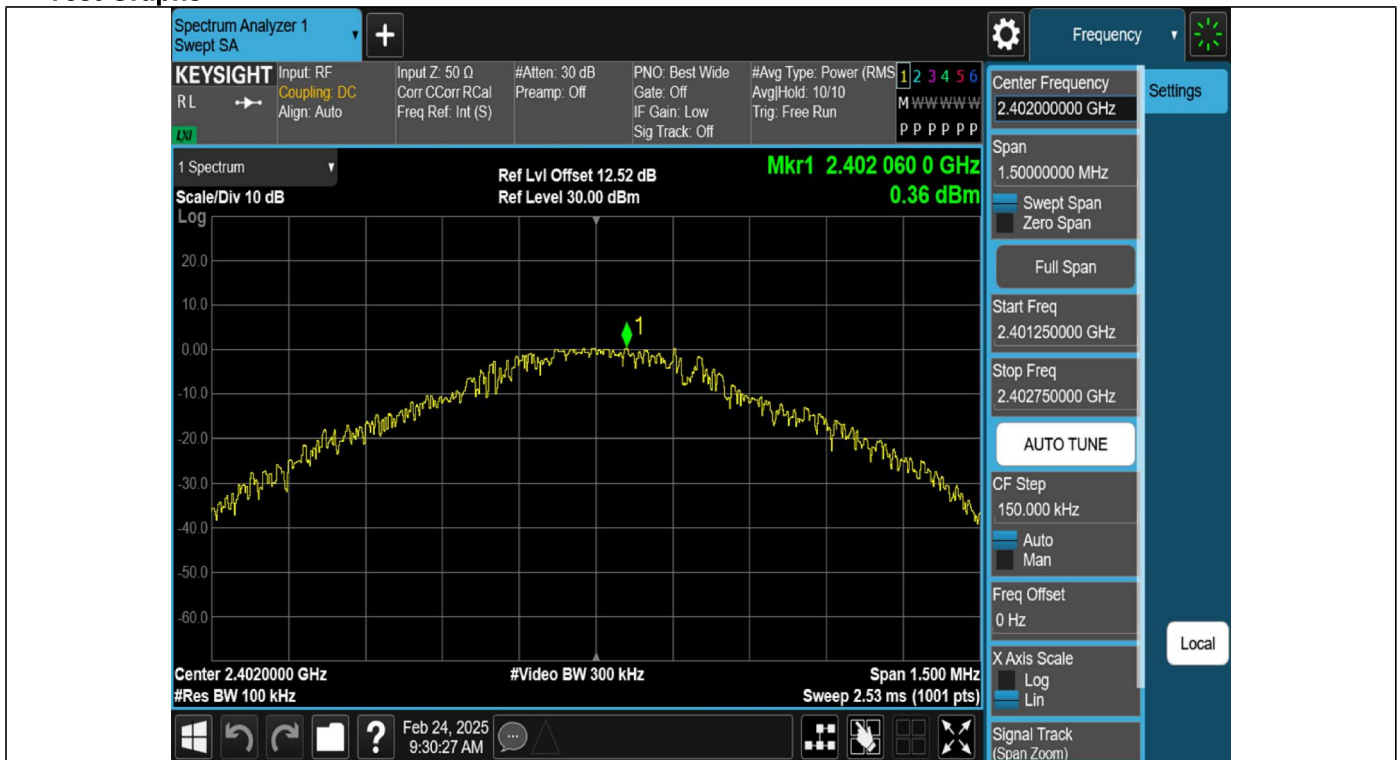
DH5-Ant1-2402-0~Reference-PASS
