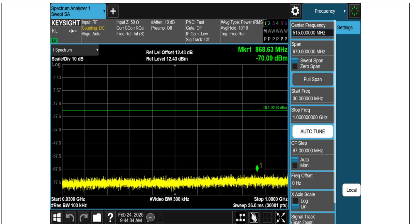
2DH5-Ant1-2480-30~1000-PASS
