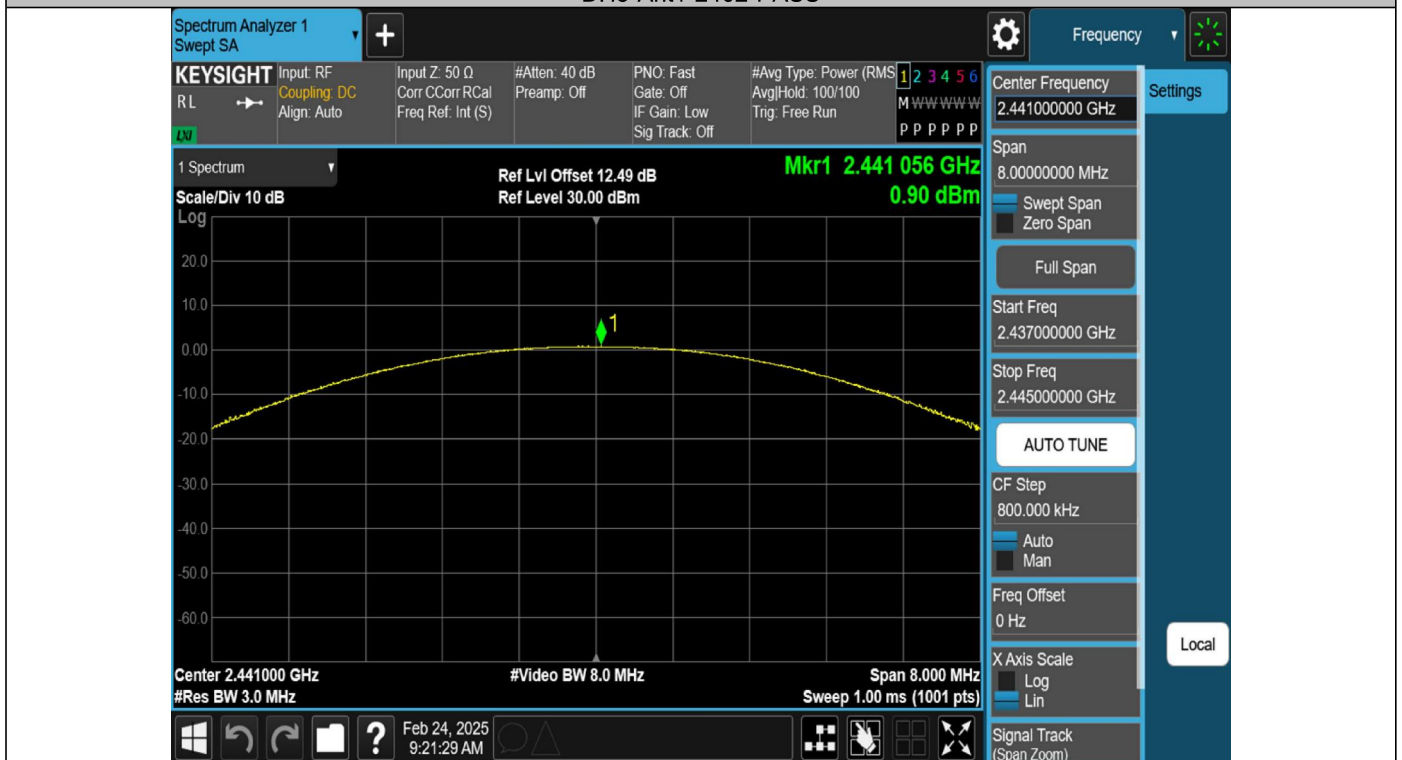
DH5-Ant1-2441-PASS
