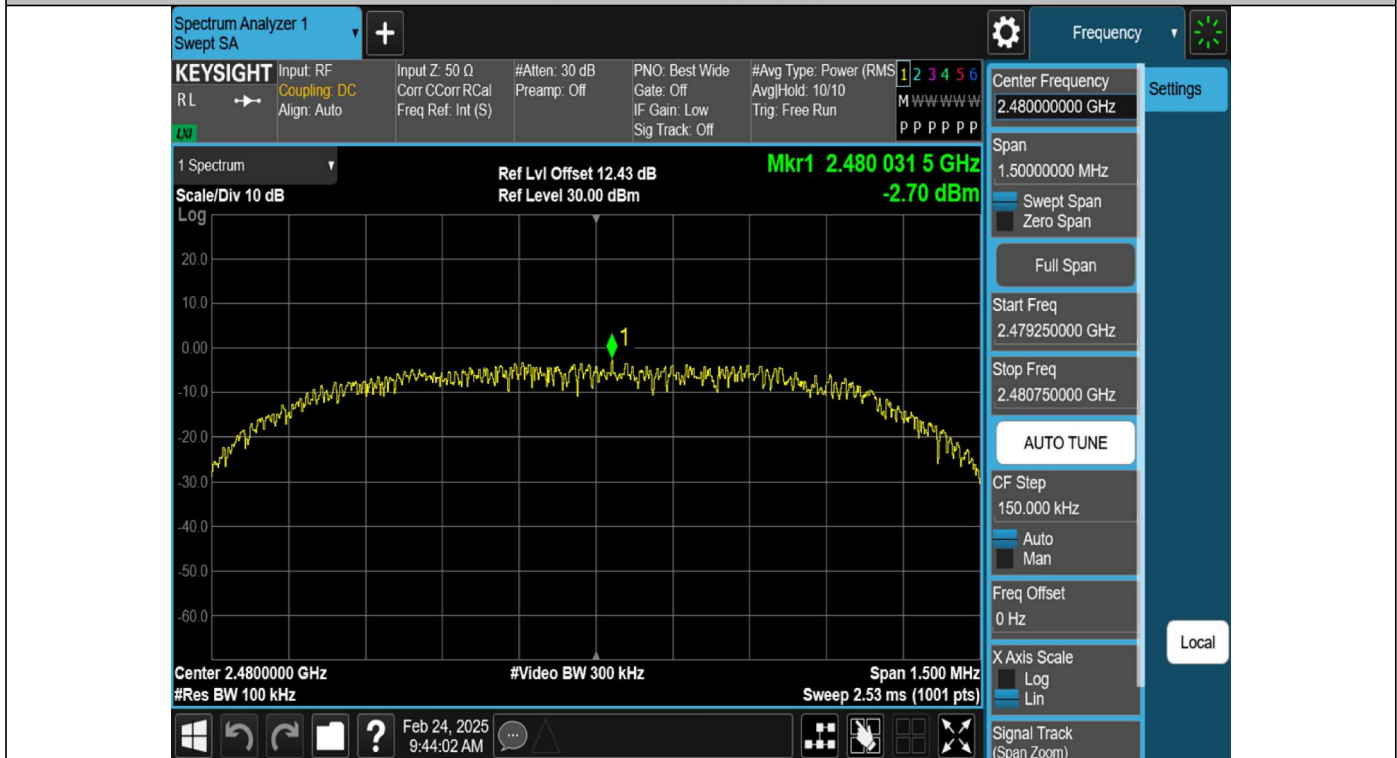
2DH5-Ant1-2480-0~Reference-PASS
