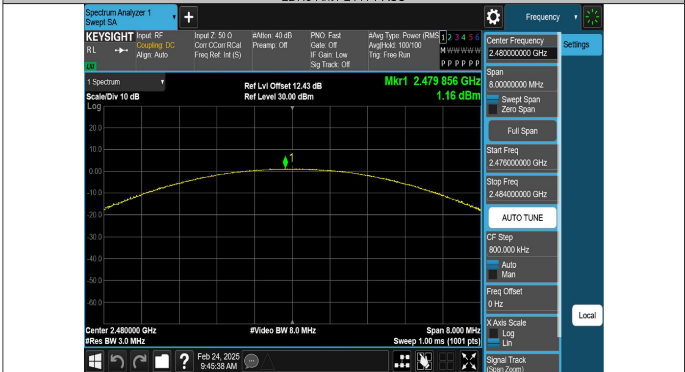
2DH5-Ant1-2480-PASS
