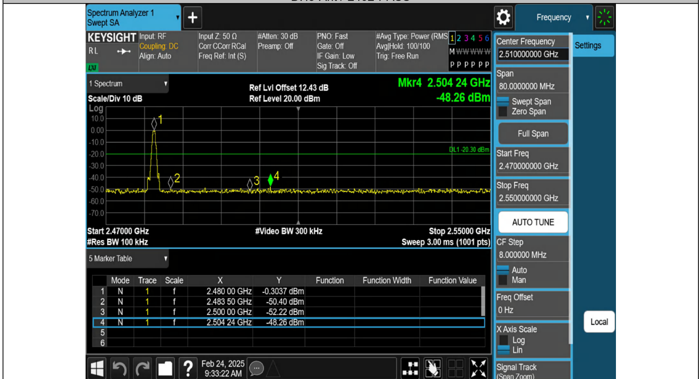
DH5-Ant1-2480-PASS
