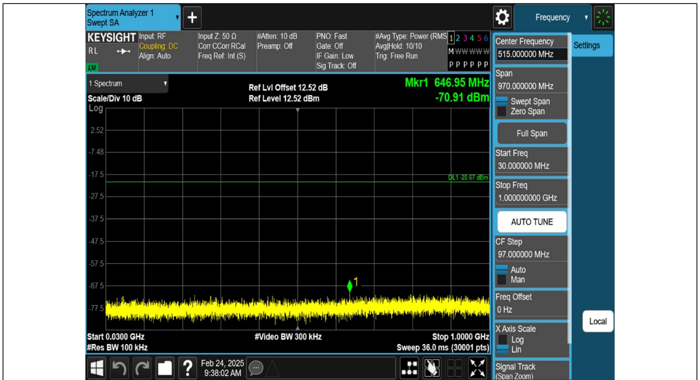
2DH5-Ant1-2402-30~1000-PASS
