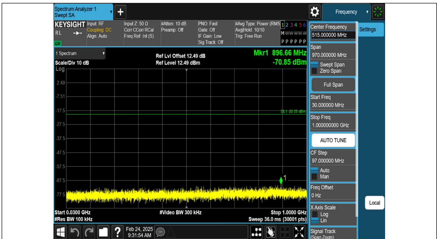
DH5-Ant1-2441-30~1000-PASS
