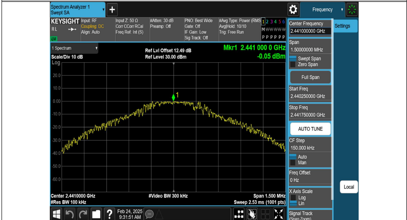
DH5-Ant1-2441-0~Reference-PASS
