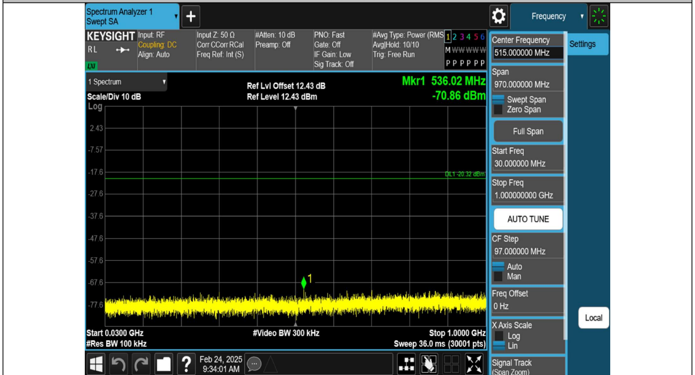
DH5-Ant1-2480-30~1000-PASS
