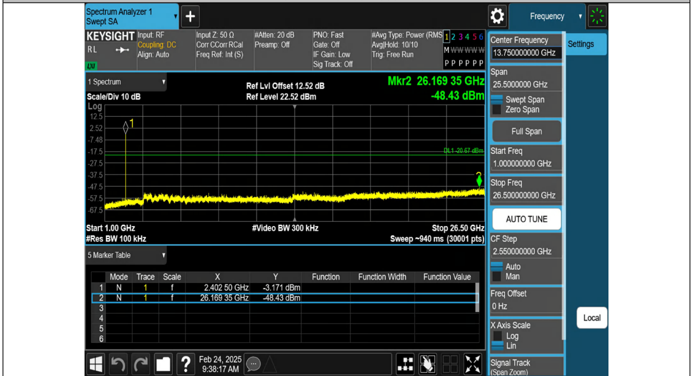
2DH5-Ant1-2402-1000~26500-PASS
