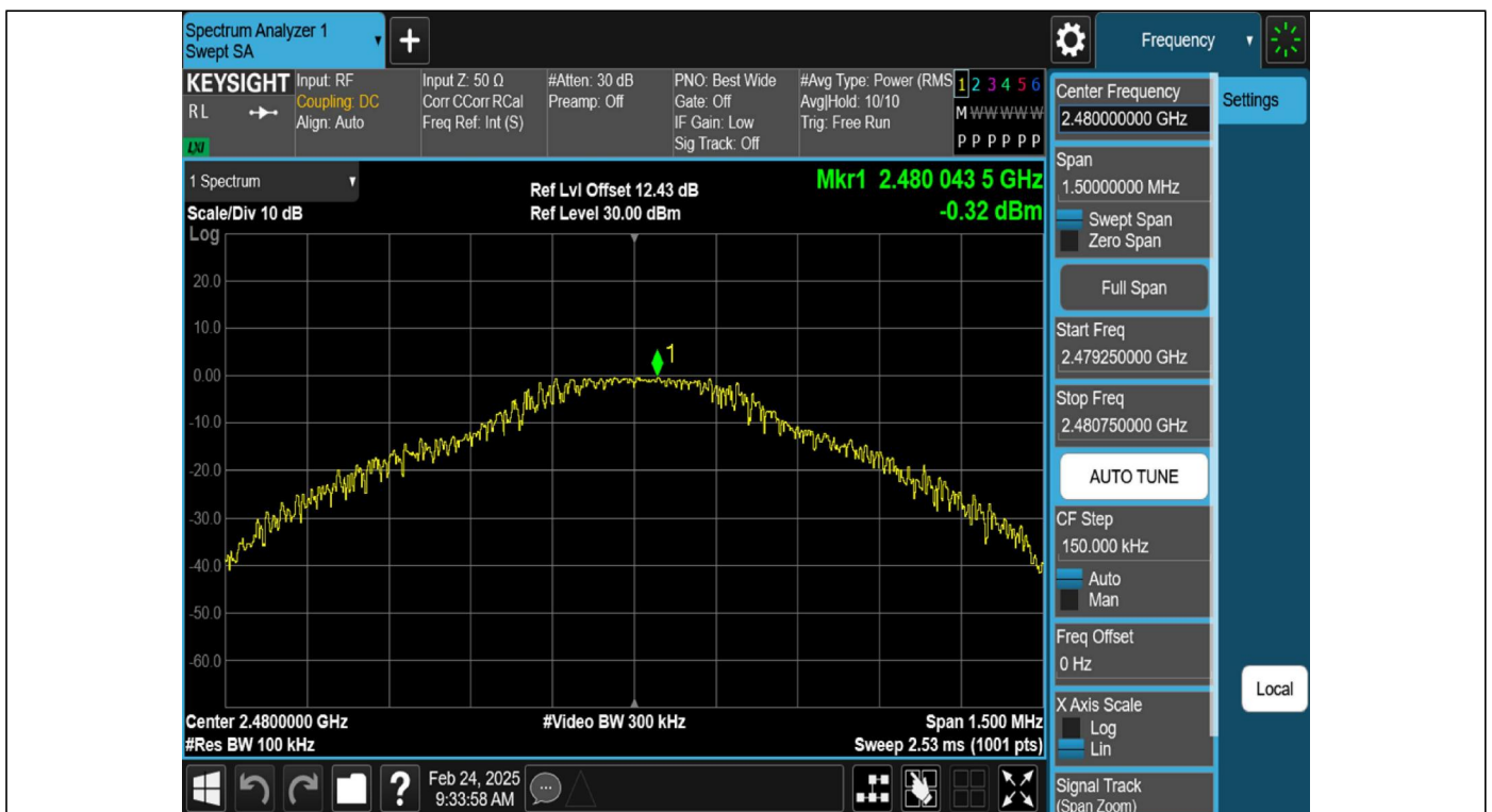
DH5-Ant1-2480-0~Reference-PASS
