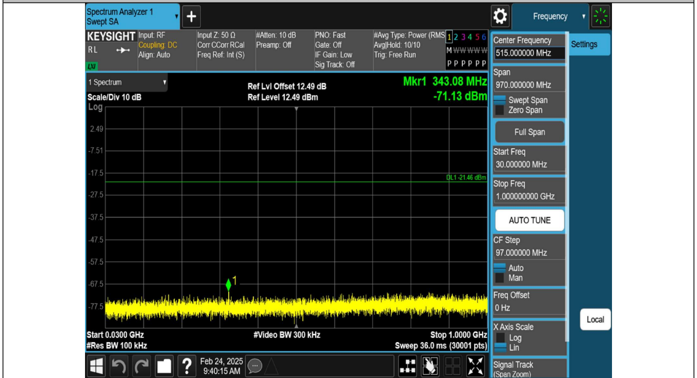
2DH5-Ant1-2441-30~1000-PASS
