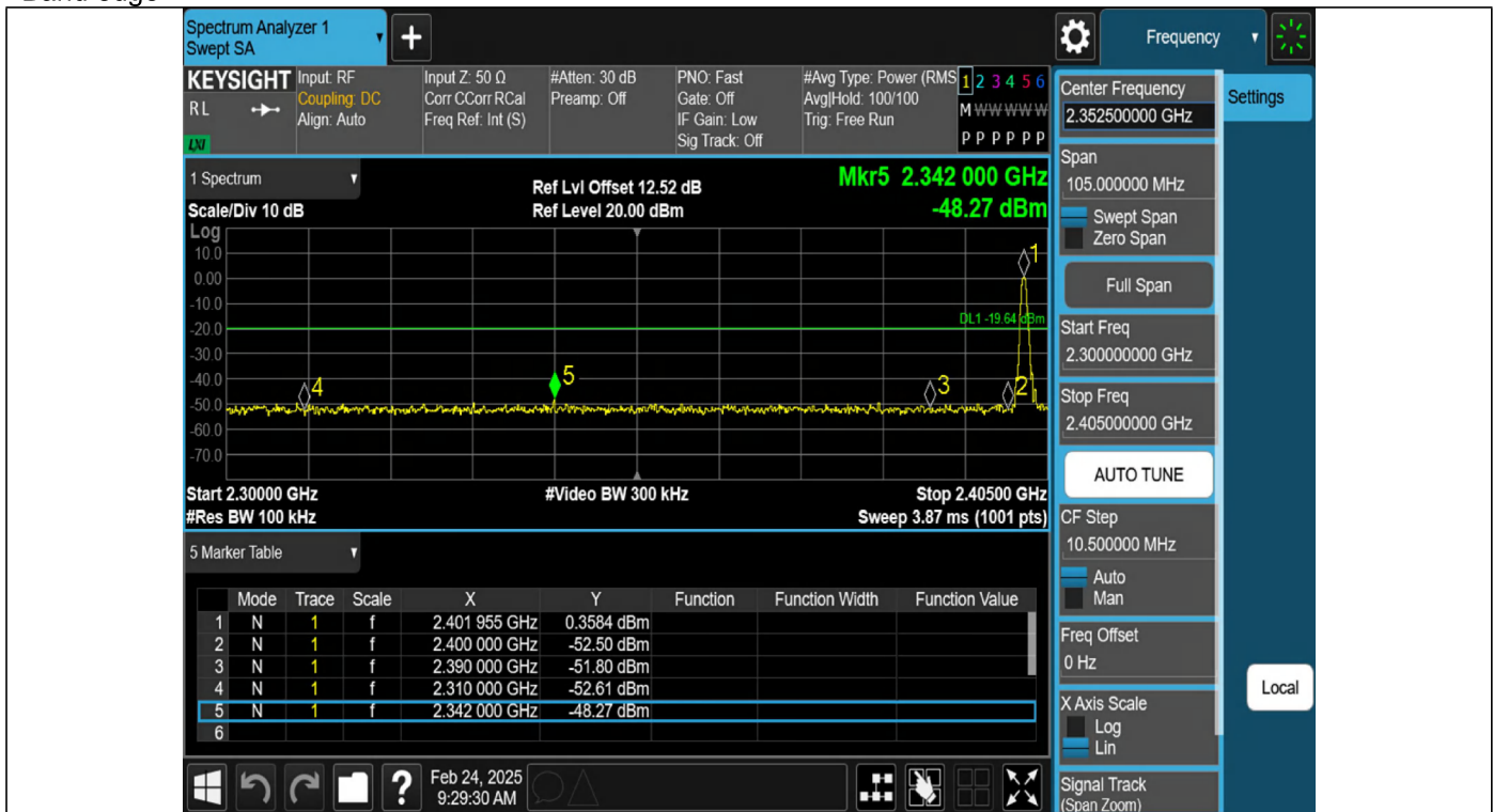
DH5-Ant1-2402-PASS
