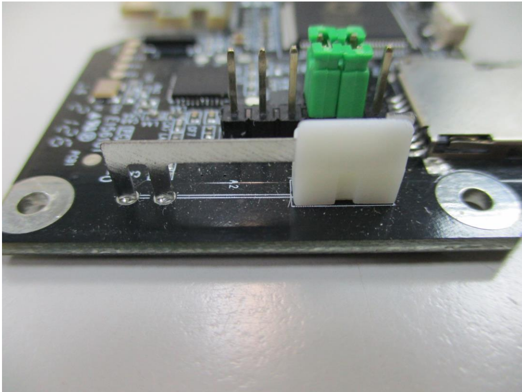
Sensor Antenna
