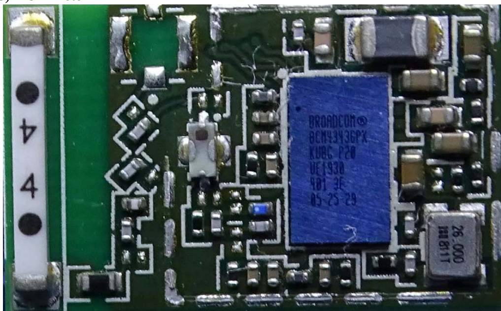
(45) EUT Photo
