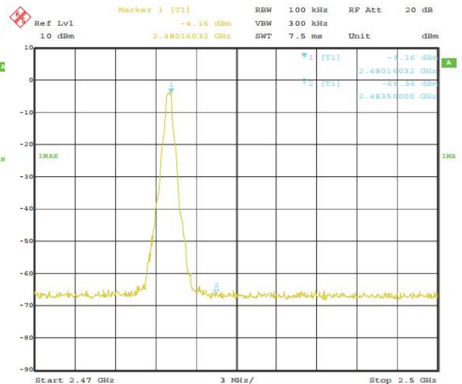
GFSK: Band Edge-High Channel
