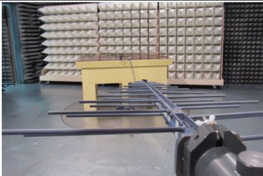
Radiated setup 2
