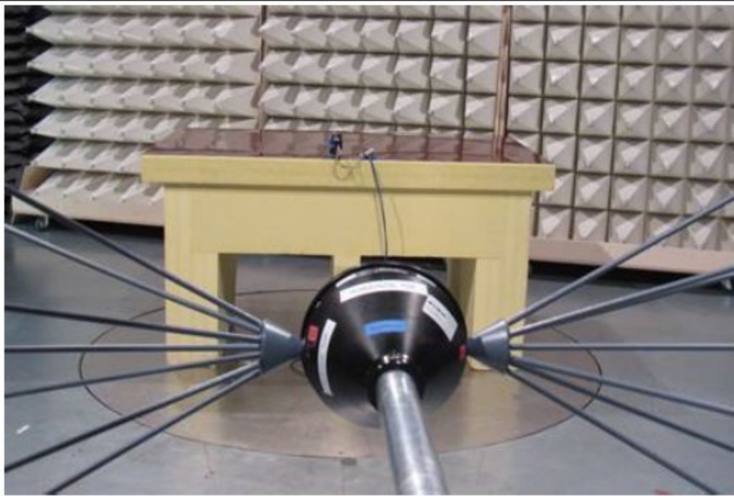
Radiated setup 2
