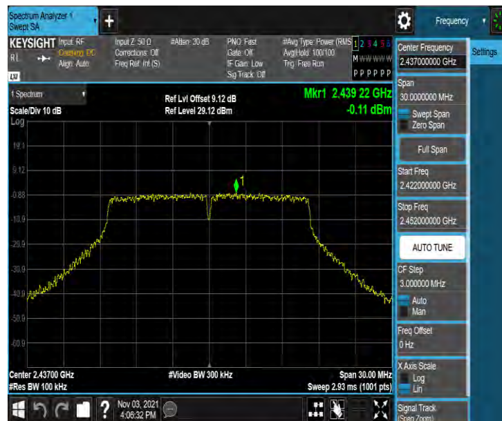
11G_Ant1_2437_0~Reference
