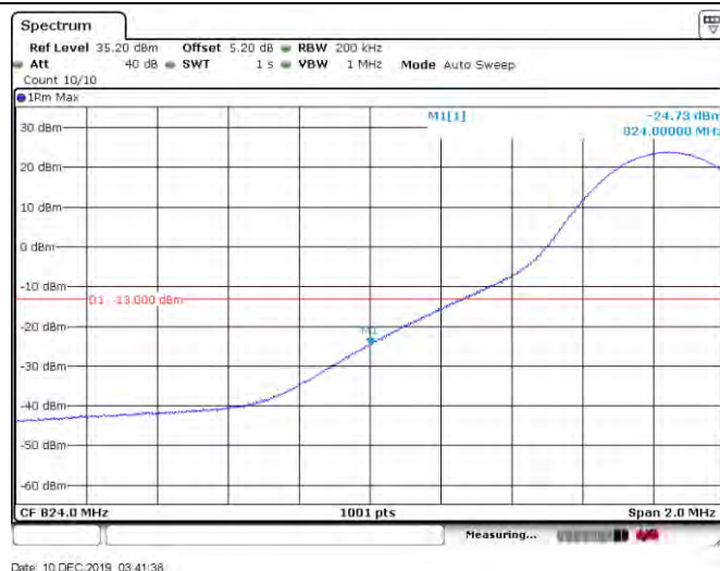
Band 26_15MHz_QPSK_26865_75RB#0
