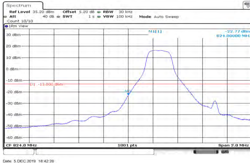
Band 26_1.4MHz_QPSK_26797_6RB#0
