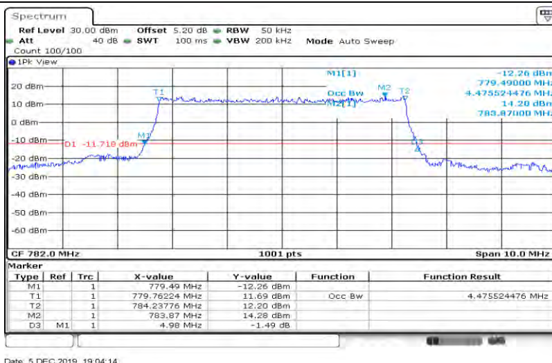
Band13-5MHz-QPSK-23255-25RB#0-4.476
