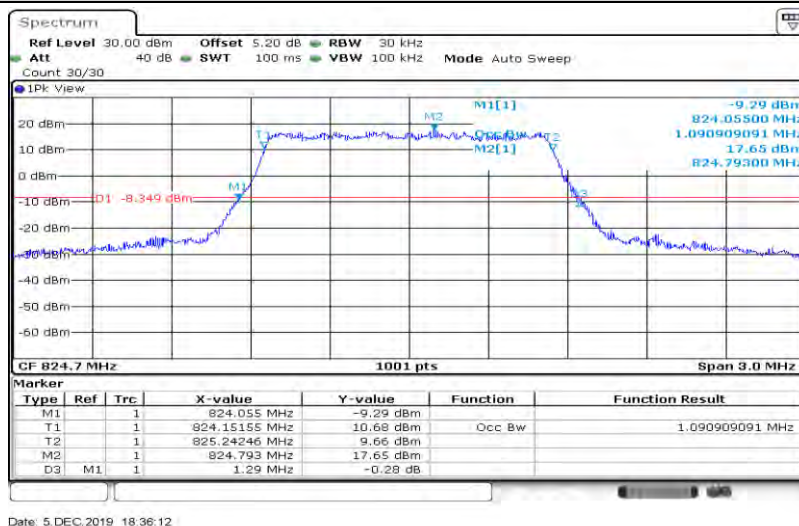
Band5-1.4MHz-QPSK-20525-6RB#0-1.091
