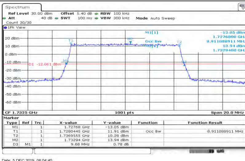
Band4-10MHz-16QAM-20350-50RB#0-8.911
