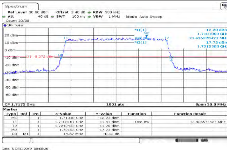
Band4-15MHz-16QAM-20175-75RB#0-13.427
