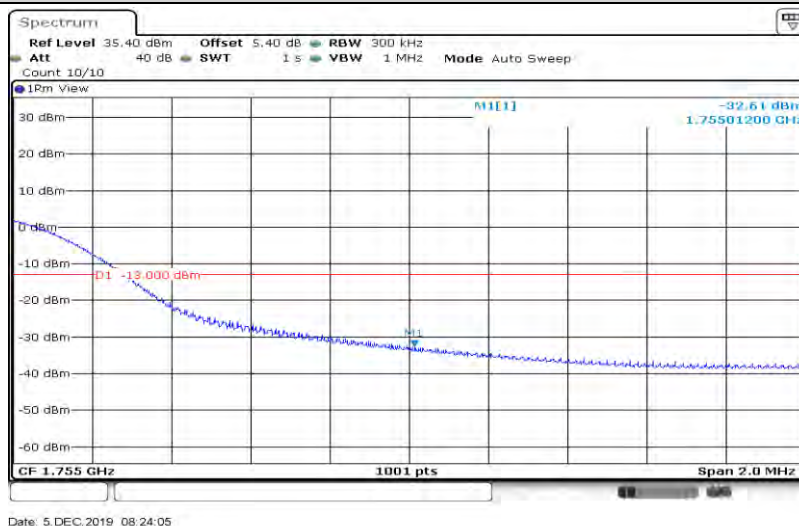
Band4-20MHz-16QAM-20050-1RB#0
