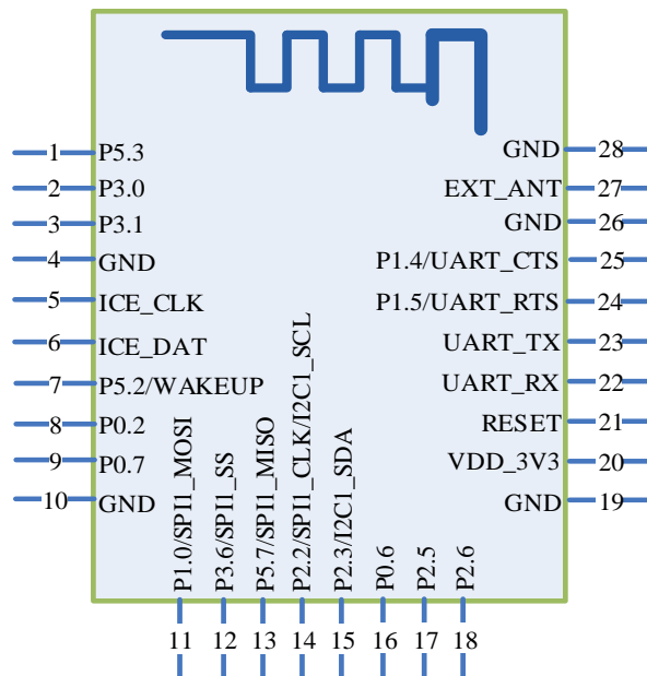
Figure 3: BT645 PIN Diagram(Top View)
