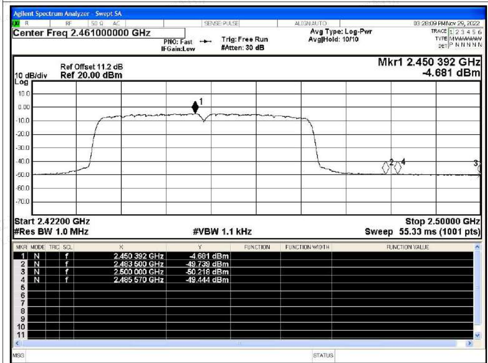
Restrict Band NVNT n40 2452MHz Average
