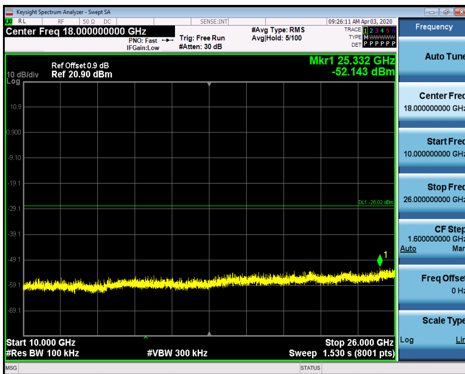
RF Conducted Spurious Emissions_2DH5_2402
