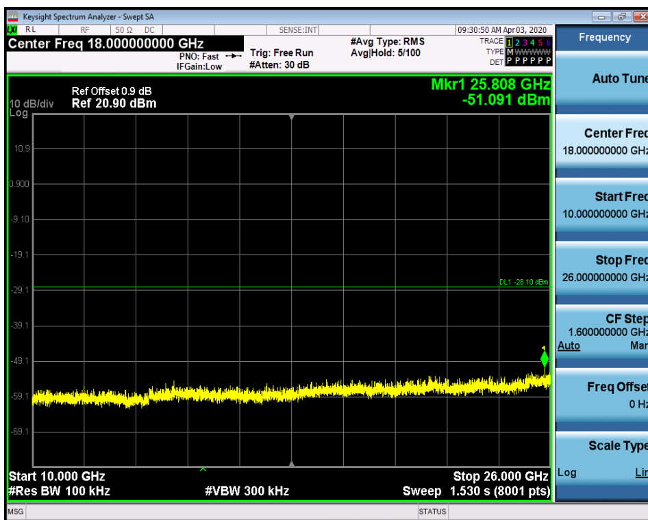
RF Conducted Spurious Emissions_2DH5_2480
